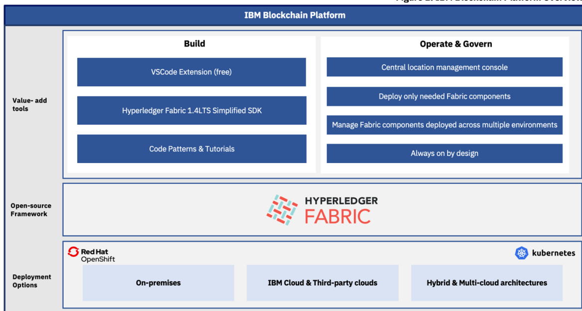
Figure 1: IBM Blockchain Platform Overview
