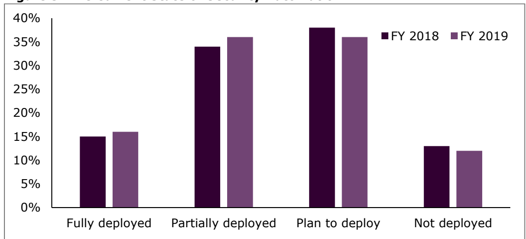
Figure 5: The Current State of Security Automation
