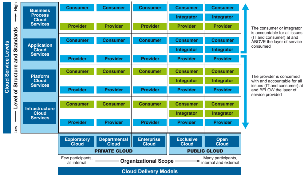
Figure 3: Roles and responsibilities. The cloud computing adoption framework defines the levels of responsibility for the provider, consumer and integrator roles in the public and private cloud models.
