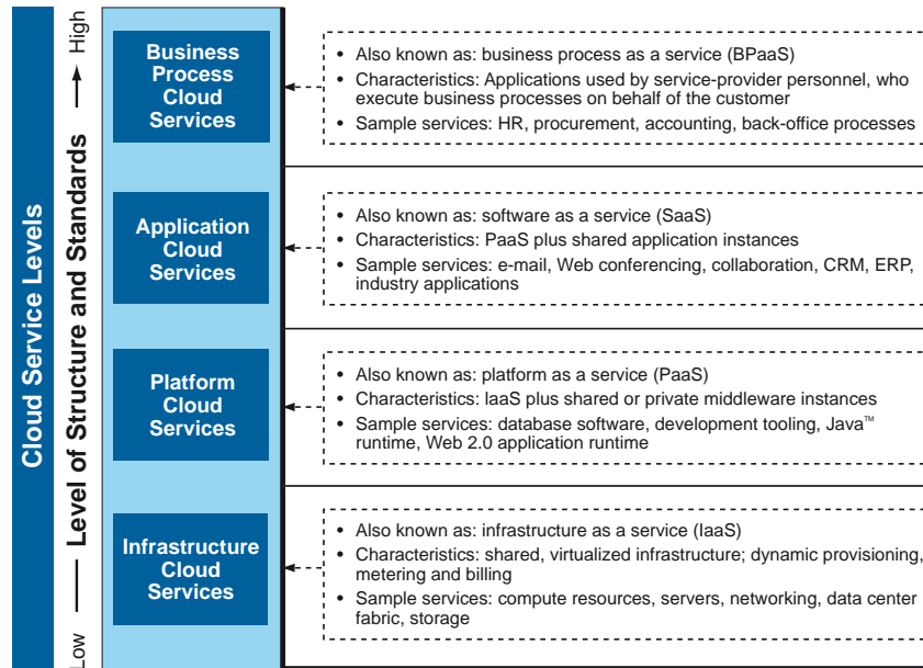
Figure 2: Cloud service types. Each type of service represents an increasing level of structure and standards, with business process cloud services requiring the most.
