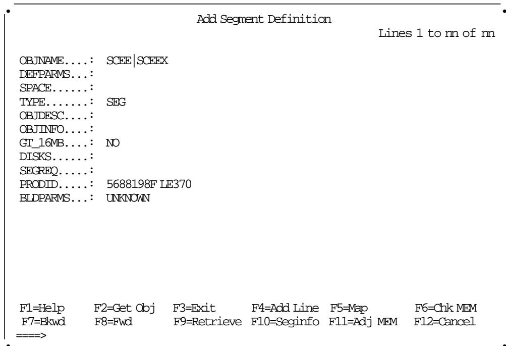
Figure 21. Initial "Add Segment Definition" panel example.
