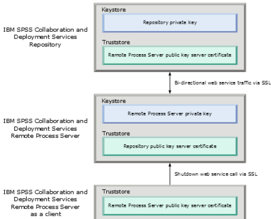
圖 1: IBM SPSS Collaboration and Deployment Services Remote Process Server 的 SSL 架構
