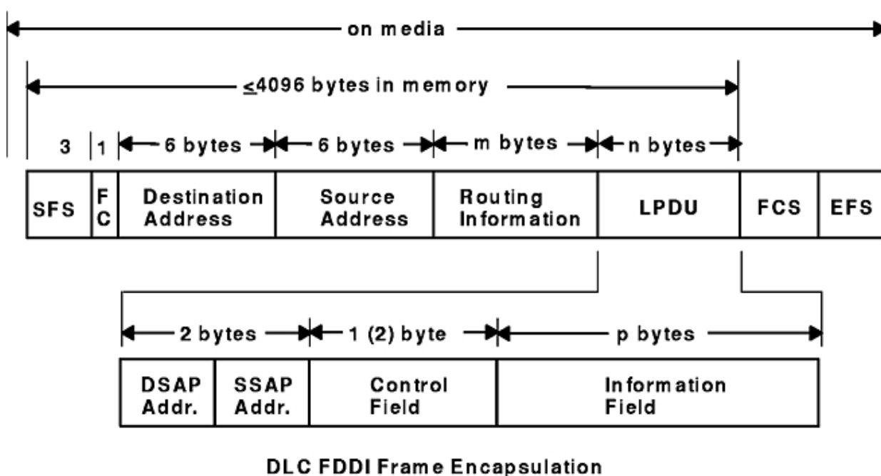
Figure 8. DLC FDDI Frame Encapsulation
