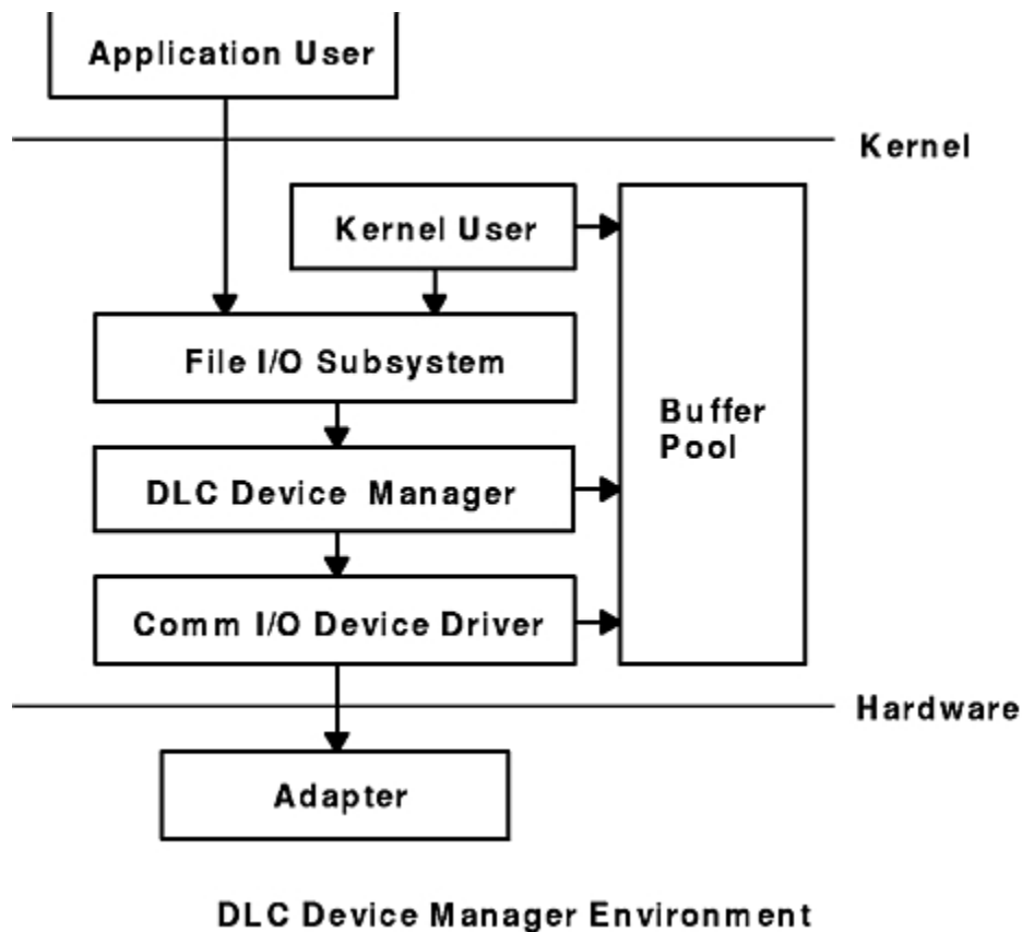
Figure 1. DLC Device Manager Environment
