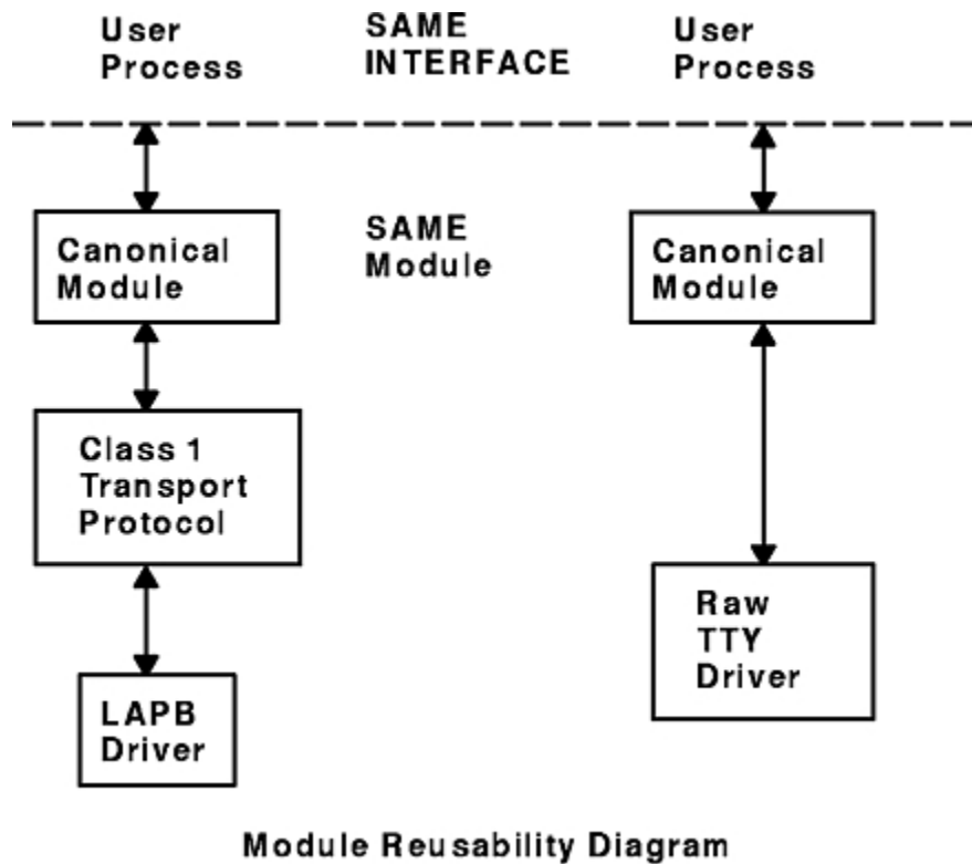
Figure 39. Module Reusability
