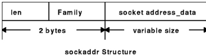
Figure 28. sockaddr Structure
