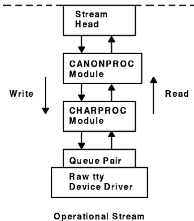
Figure 44. Operational Stream
