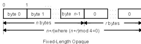
Figure 14. Fixed-Length Opaque
