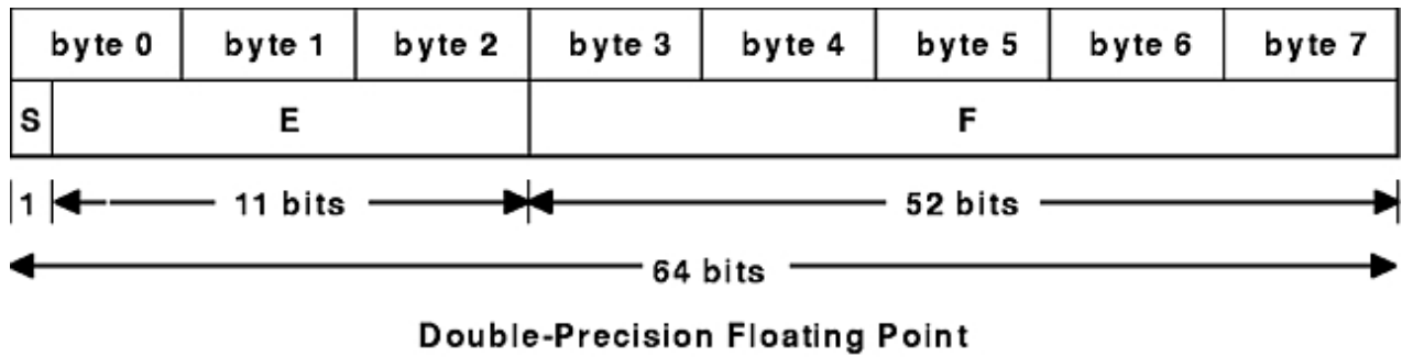
Figure 13. Double-Precision Floating-Point
