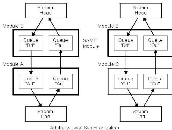
Figure 35. Arbitrary-Level Synchronization
