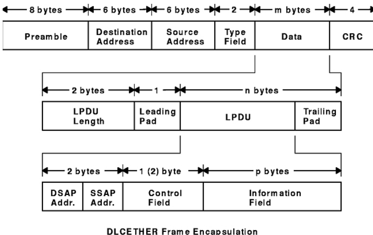
Figure 7. DLCETHER Frame Encapsulation
