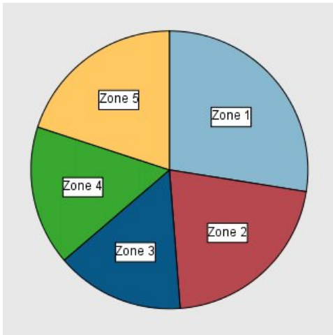
Figure 13. Pie chart
