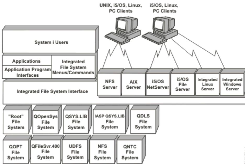
Figure 97. File systems, file servers, and the integrated file system interface
