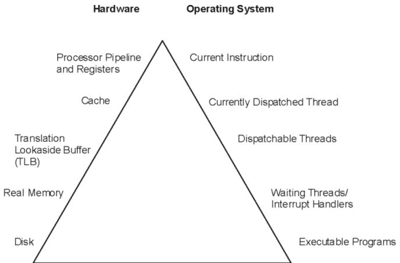
Figure 1. Program Execution Hierarchy
