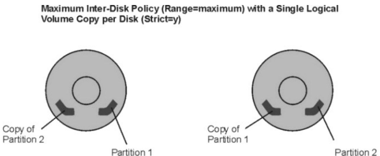
Figure 18. Inter-Physical Volume Allocation Policy
