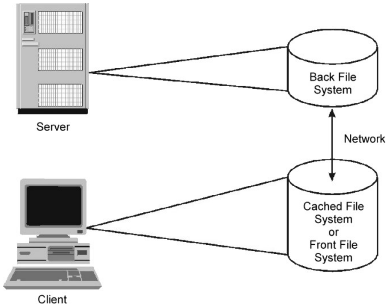
Figure 24. Cache File System (CacheFS)
