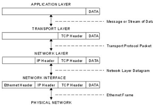
Figure 7. Host data transmissions and receptions
