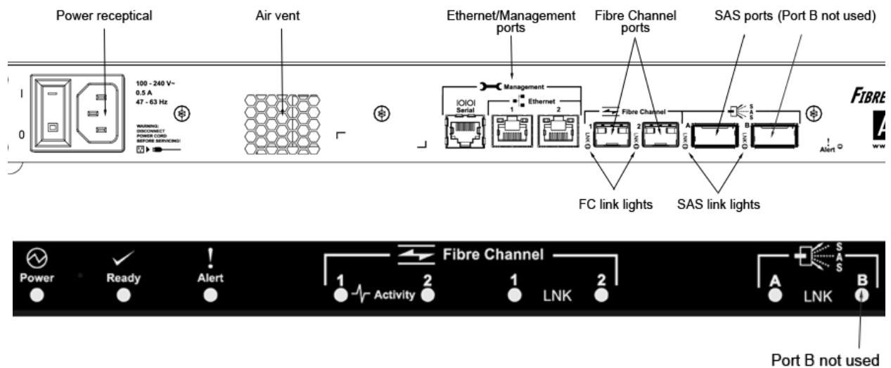
Exhibit 1.1-1 Connectors, LEDs and power receptacle on the connector side and LEDs on the faceplate.
