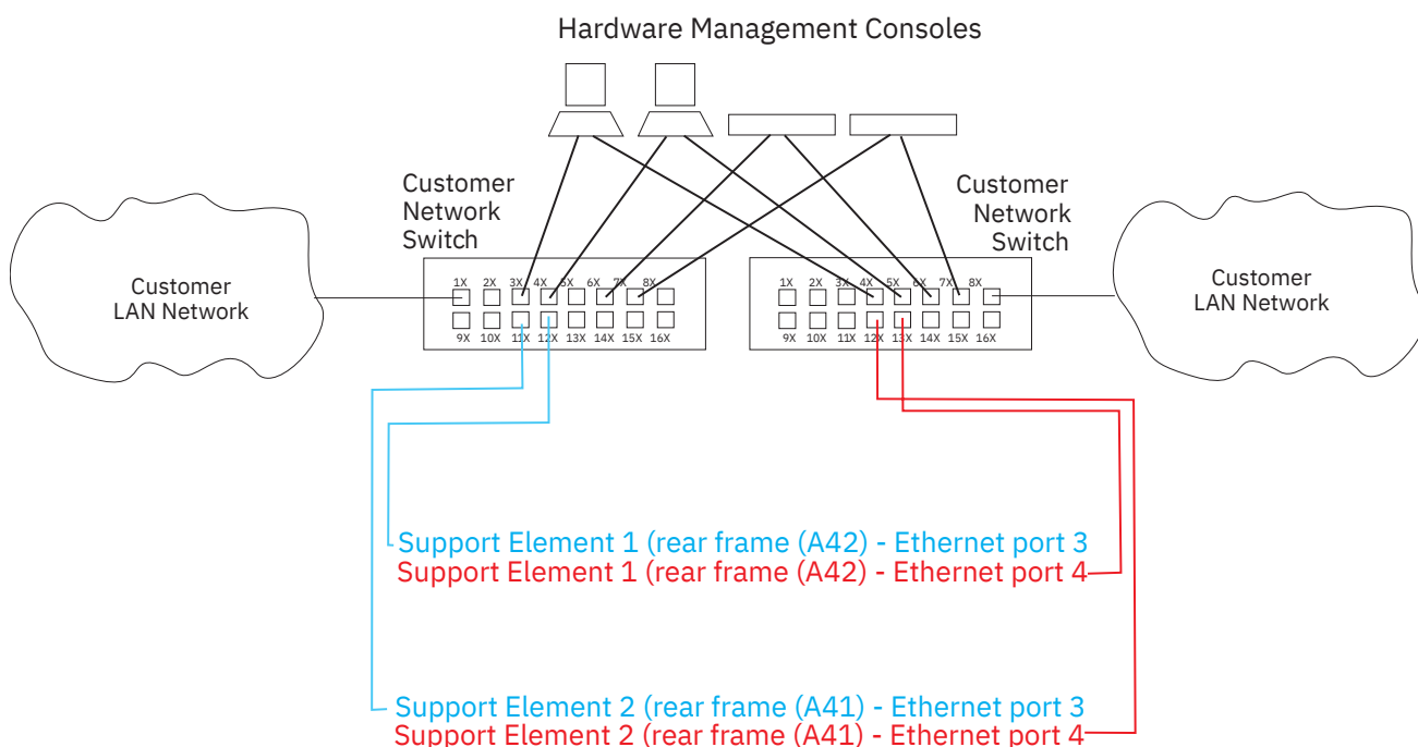
Figure 32. Two-switch configuration
