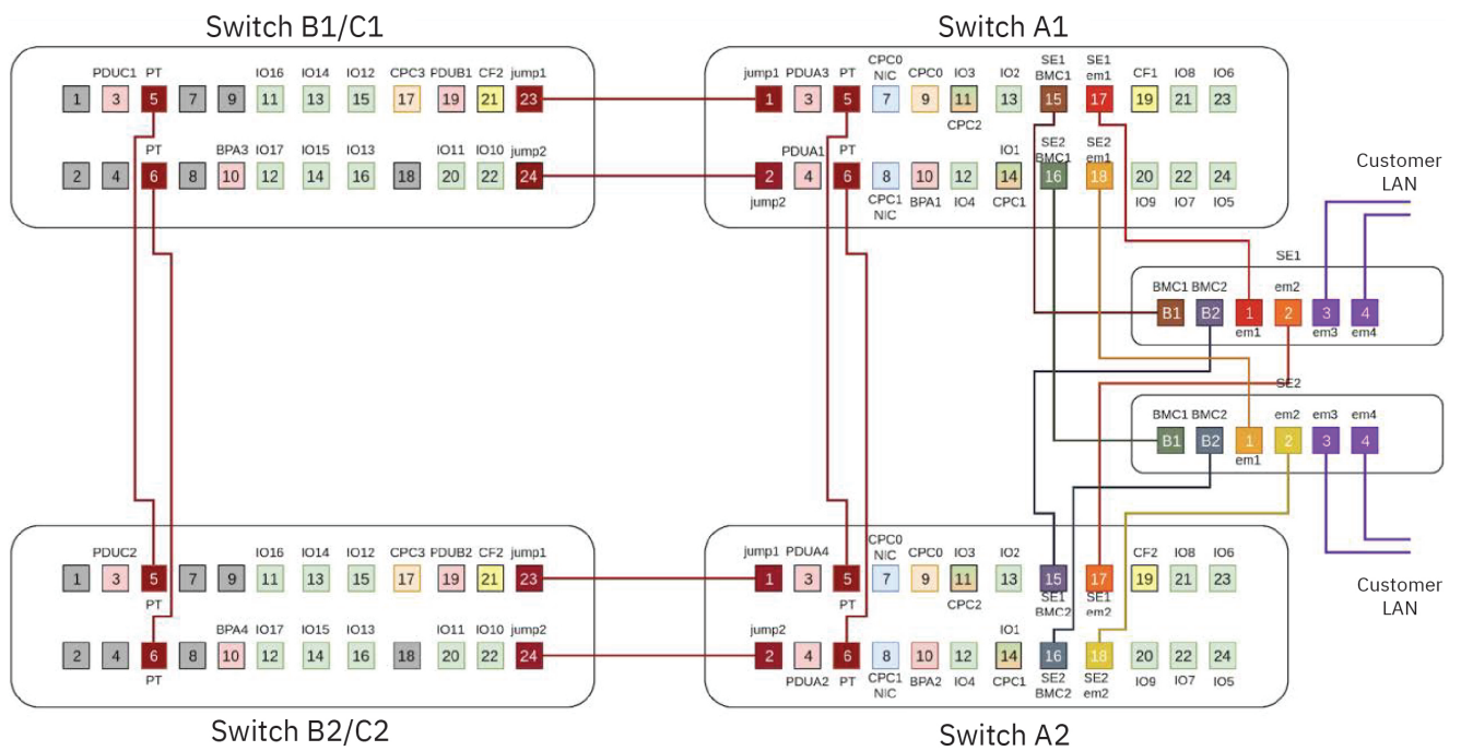
Figure 34. Ethernet Switch assignments
