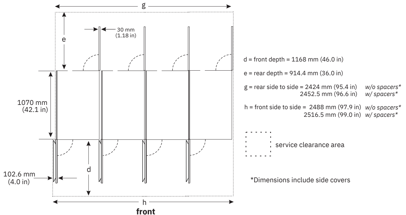
Figure 17. Maximum service clearance area (four frames)
