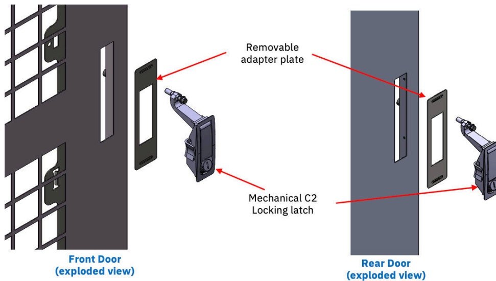
Figure 22. Front and rear door latches
