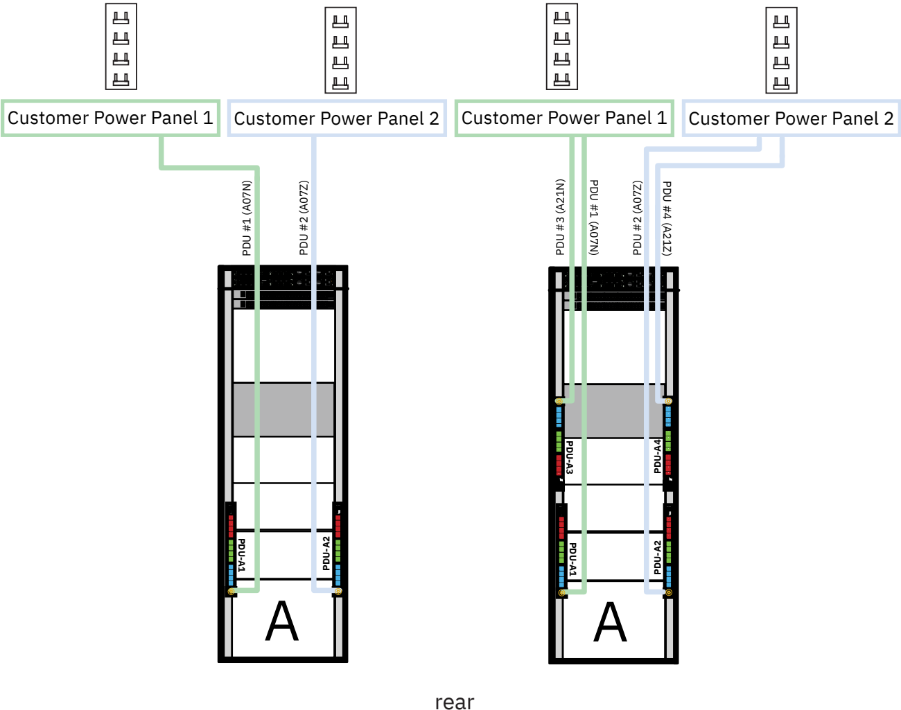
Figure 53. A frame
