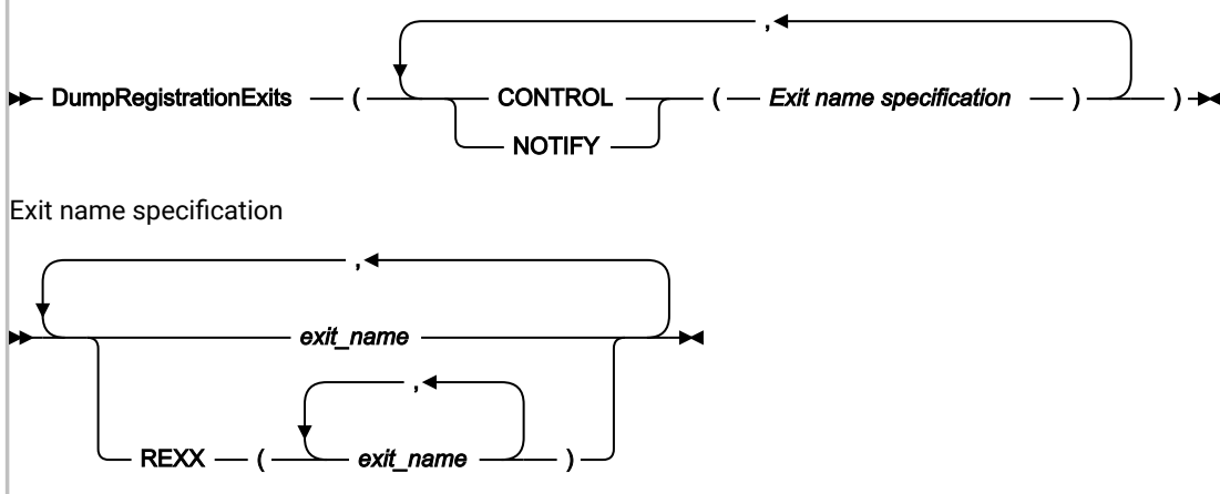
Figure 300. Syntax
