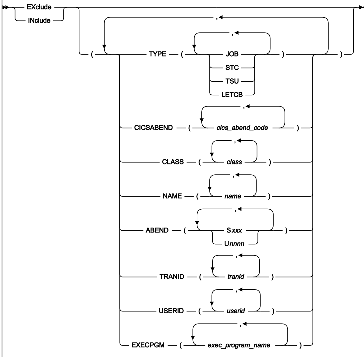
Figure 302. Syntax
