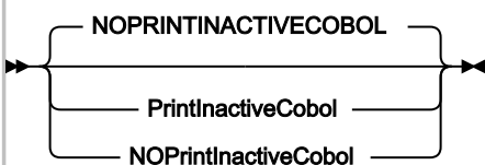
Figure 330. Syntax
