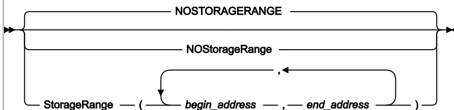
Figure 339. Syntax
