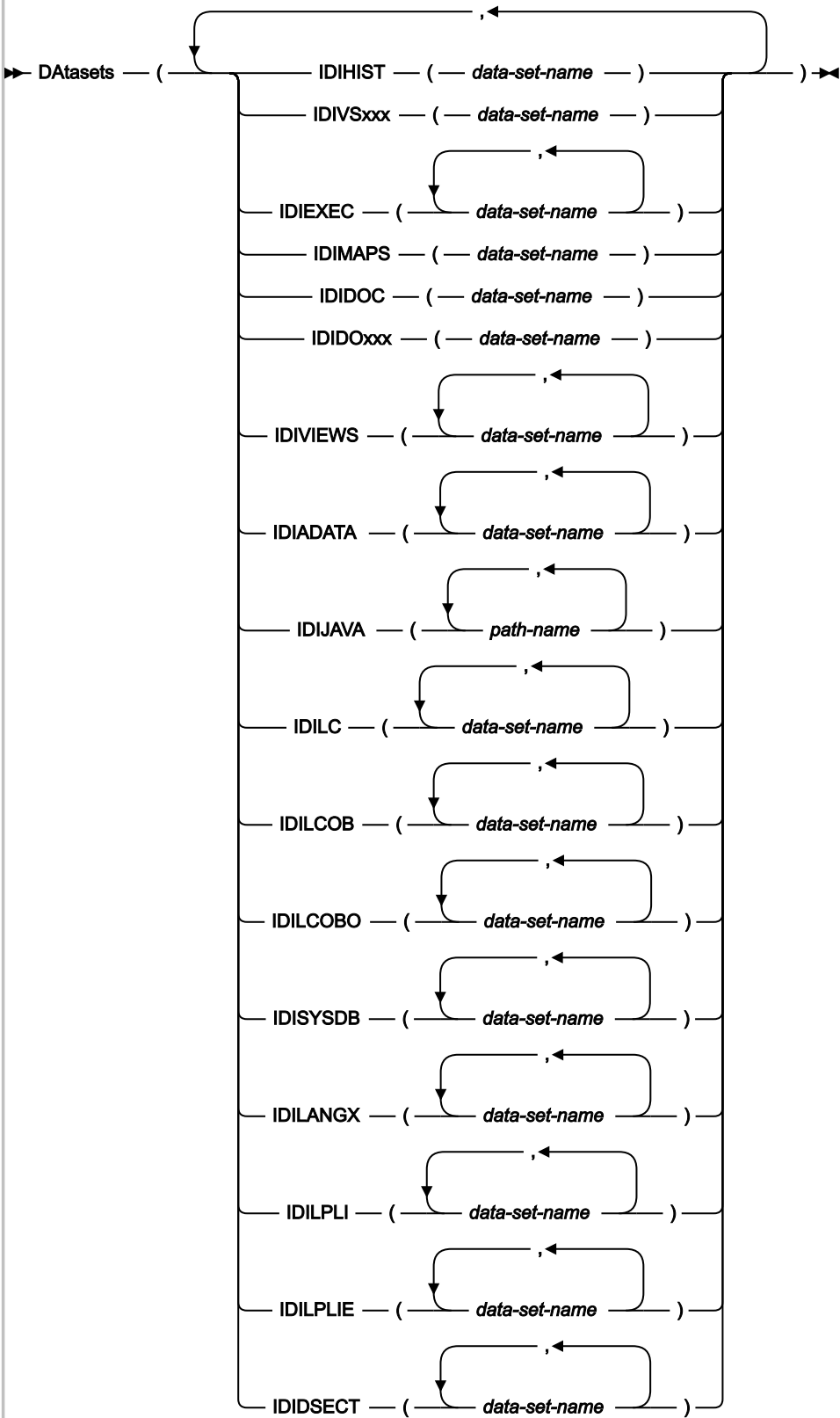
Figure 295. Syntax
