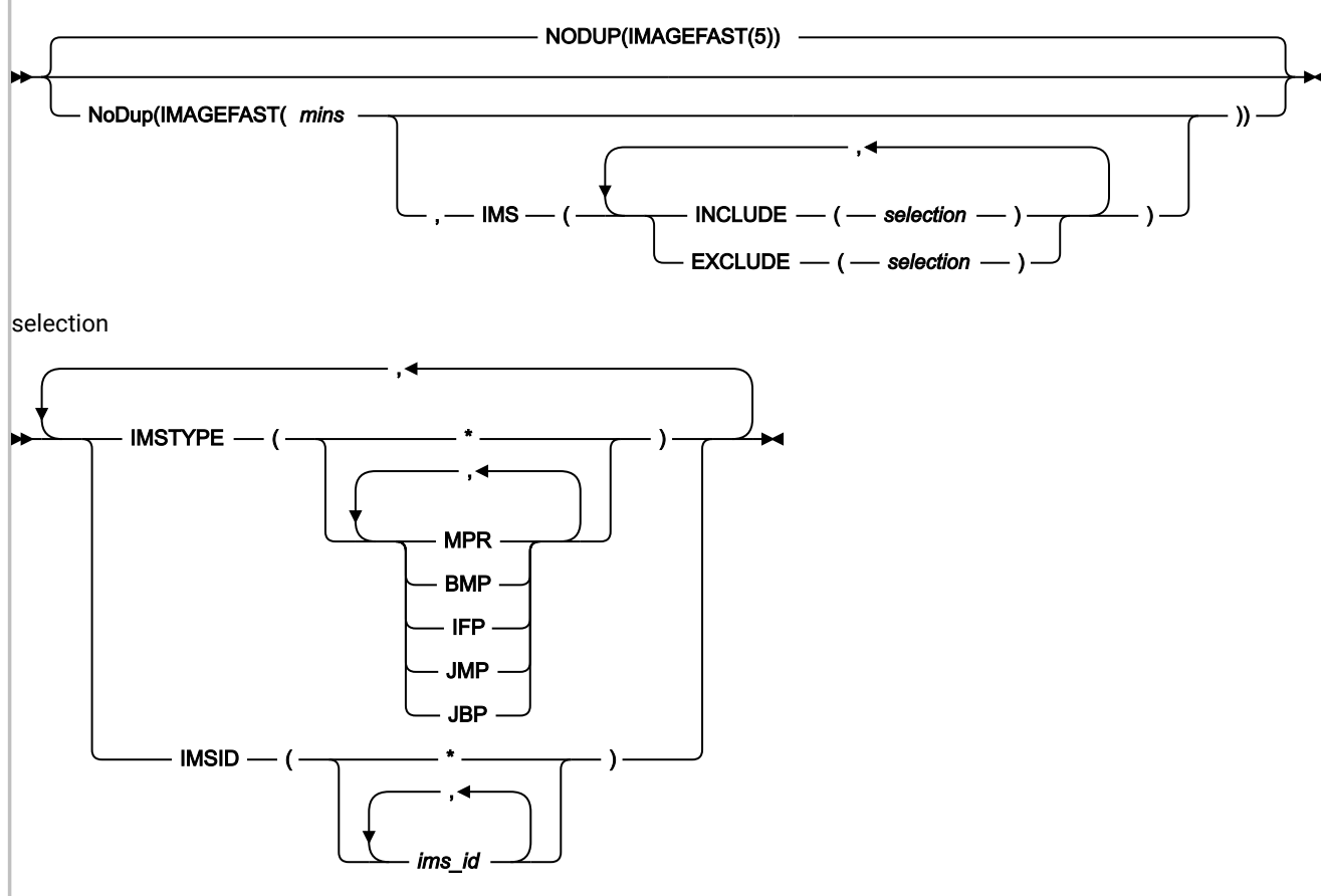
Figure 323. Syntax
