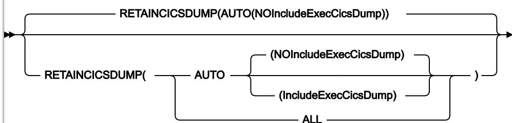
Figure 333. Syntax
