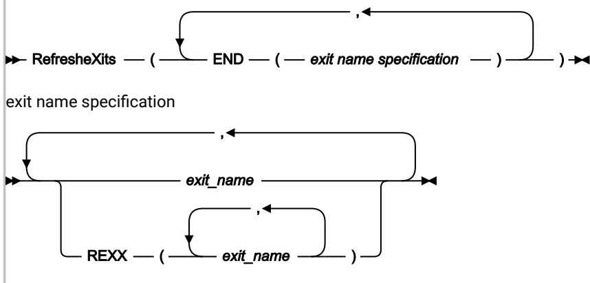
Figure 332. Syntax
