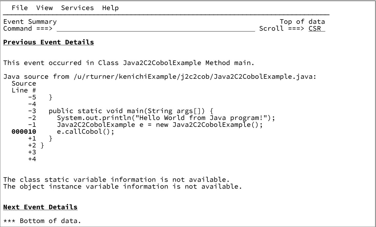
Figure 180. Sample Java Event Details display
