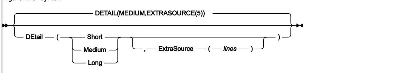
Figure 298. Syntax
