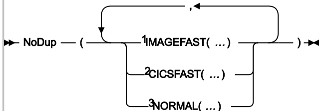
Figure 322. Syntax
