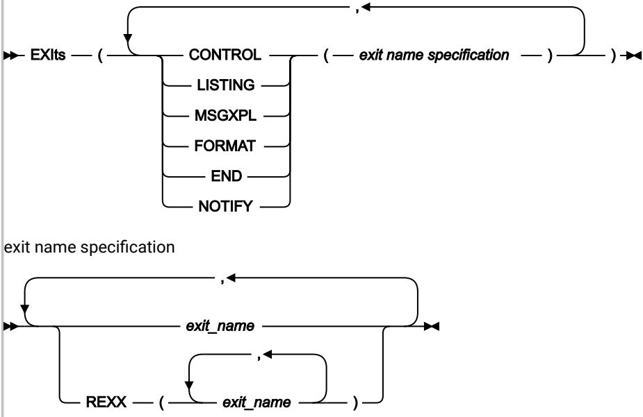
Figure 304. Syntax
