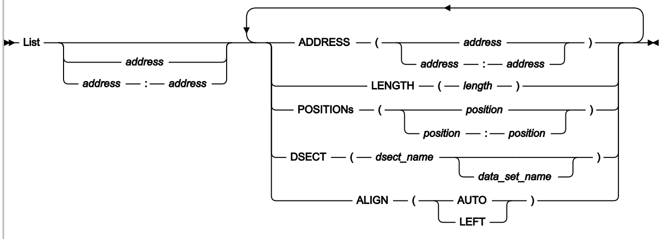
Figure 267. Syntax
