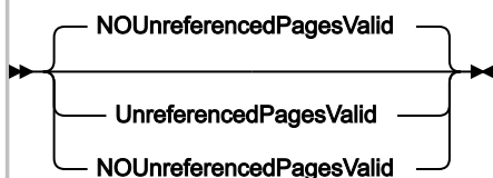
Figure 341. Syntax
