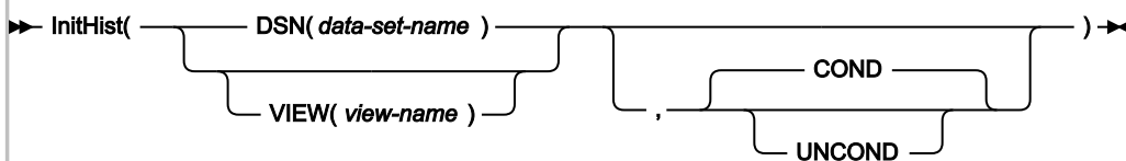
Figure 312. Syntax
