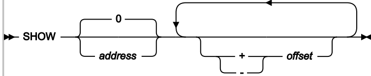
Figure 54. Syntax
