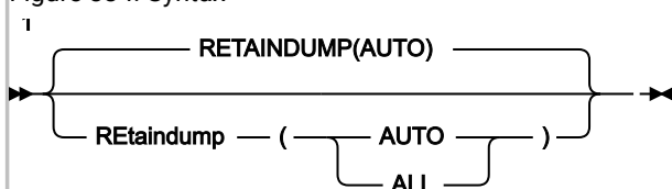
Figure 334. Syntax
