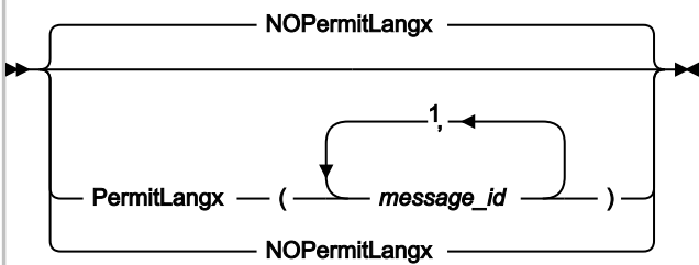
Figure 328. Syntax
