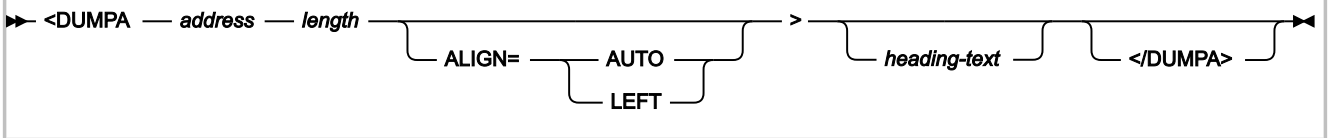
Figure 280. Syntax
