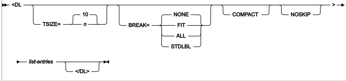
Figure 277. Syntax
