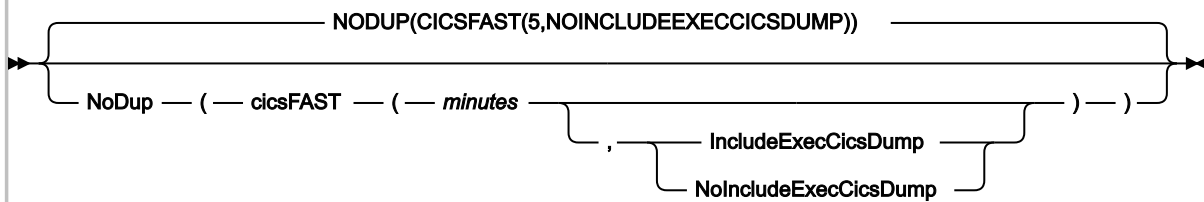
Figure 324. Syntax
