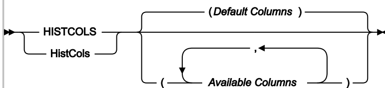
Figure 311. Syntax
