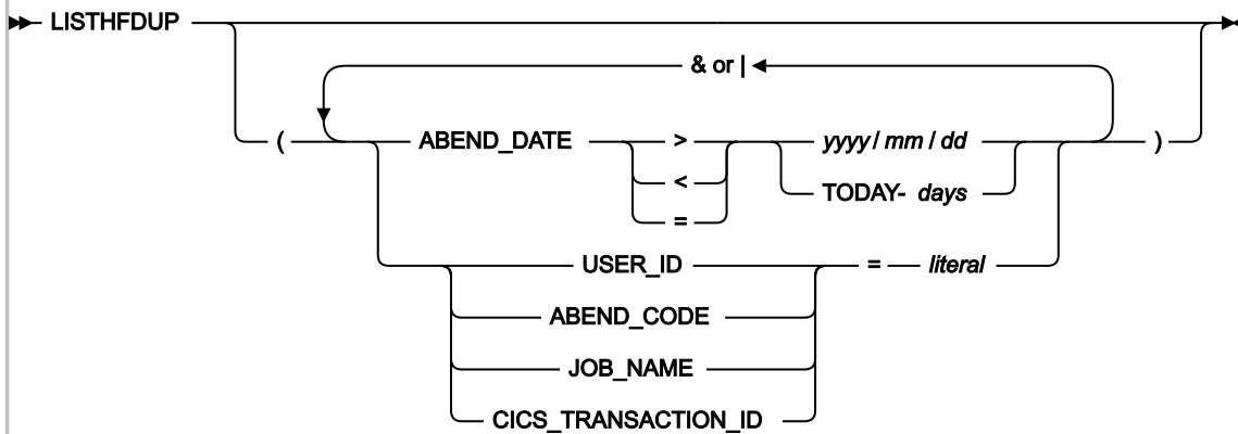
Figure 214. Syntax
