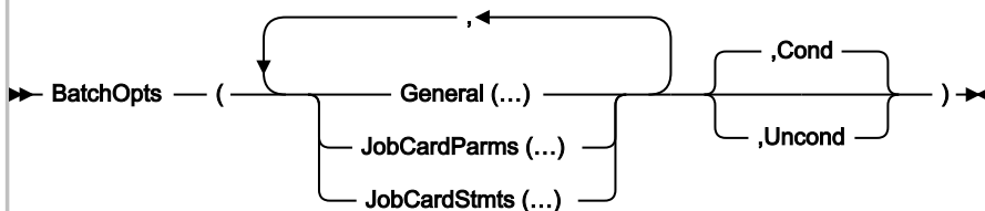
Figure 306. Syntax
