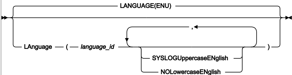
Figure 317. Syntax
