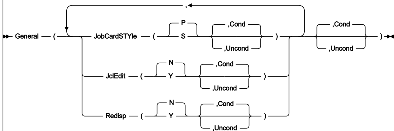
Figure 307. Syntax
