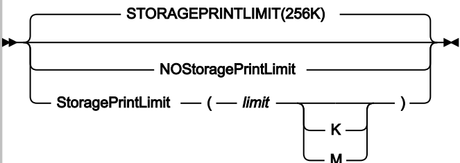
Figure 338. Syntax
