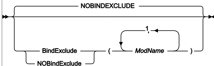
Figure 291. Syntax
