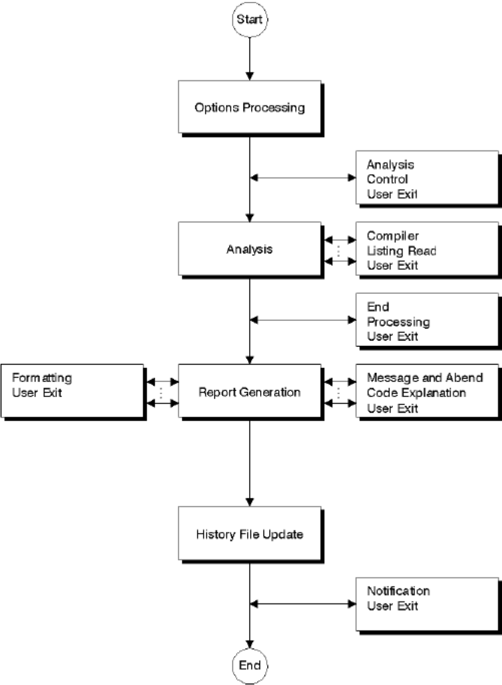
Figure 225. Fault Analyzer analysis exit points (IDIDA)
