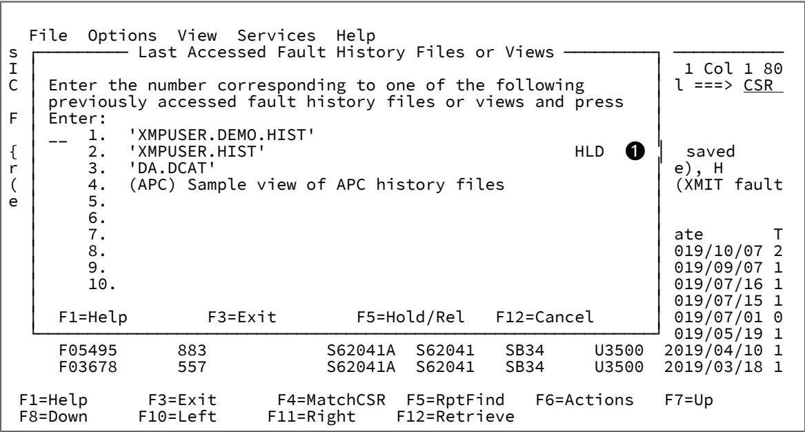
Figure 11. Sample Last Accessed Fault History Files or Views display
