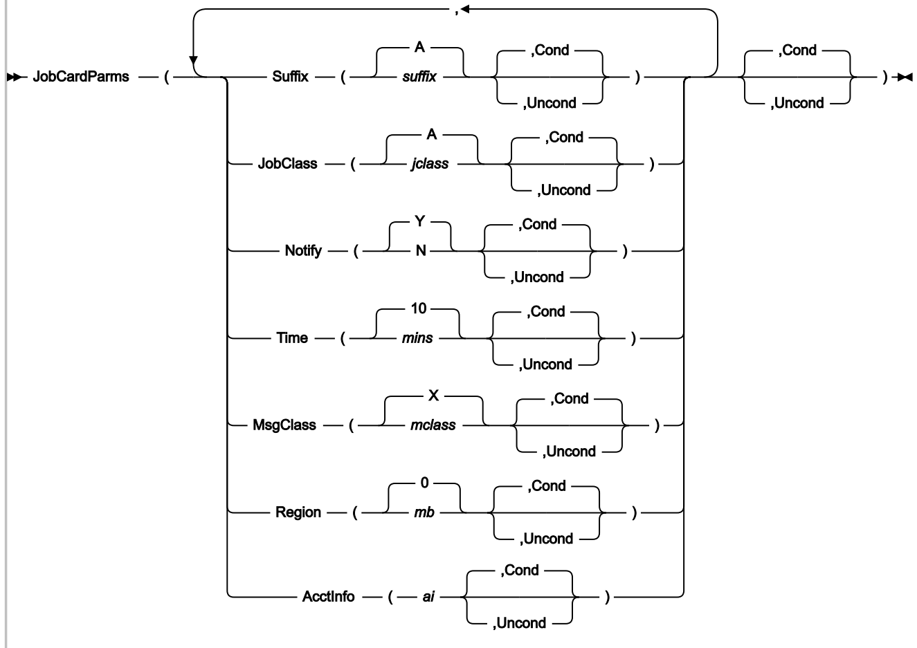
Figure 305. Syntax
