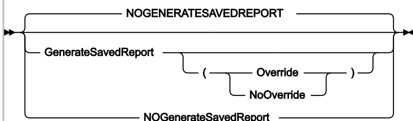
Figure 312. Syntax
