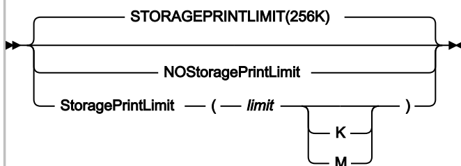
Figure 335. Syntax
