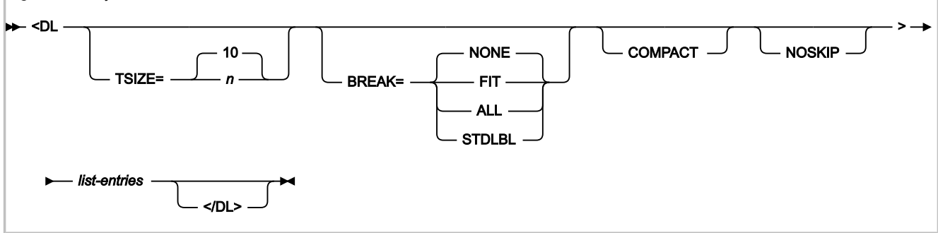
Figure 275. Syntax
