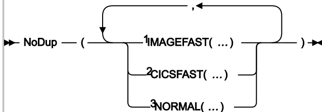
Figure 319. Syntax
