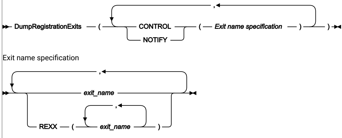
Figure 297. Syntax
