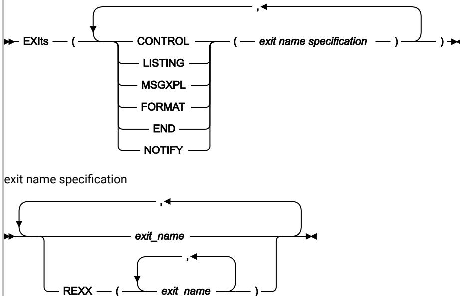
Figure 301. Syntax
