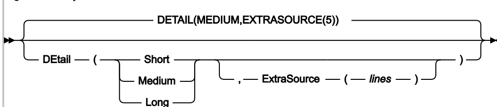
Figure 295. Syntax
