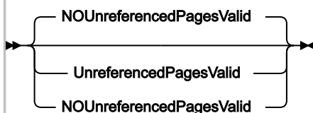
Figure 338. Syntax
