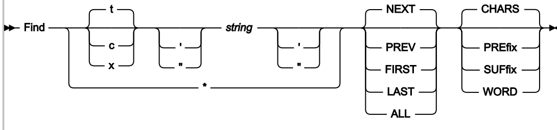
Figure 39. Syntax
