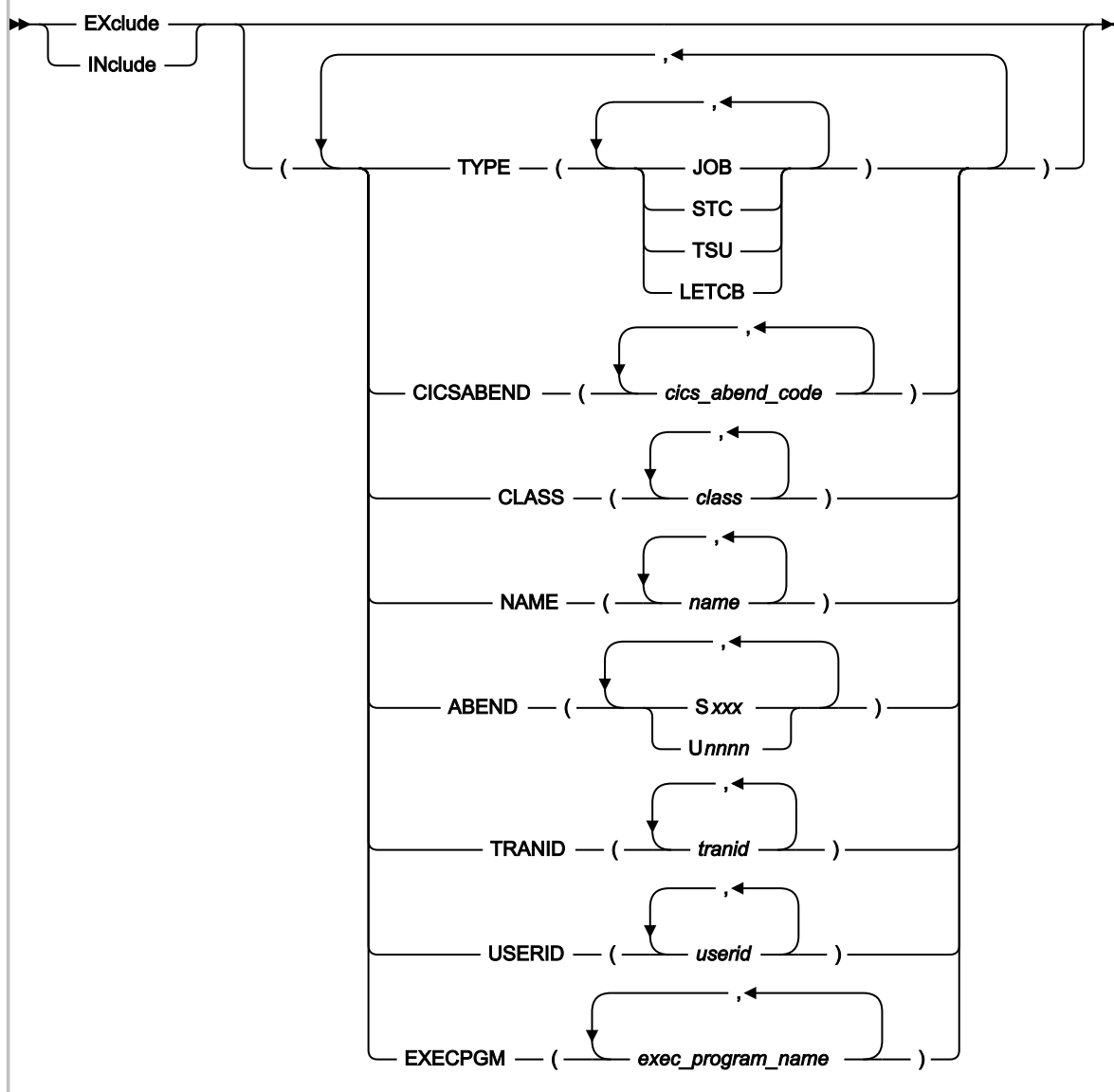
Figure 299. Syntax
