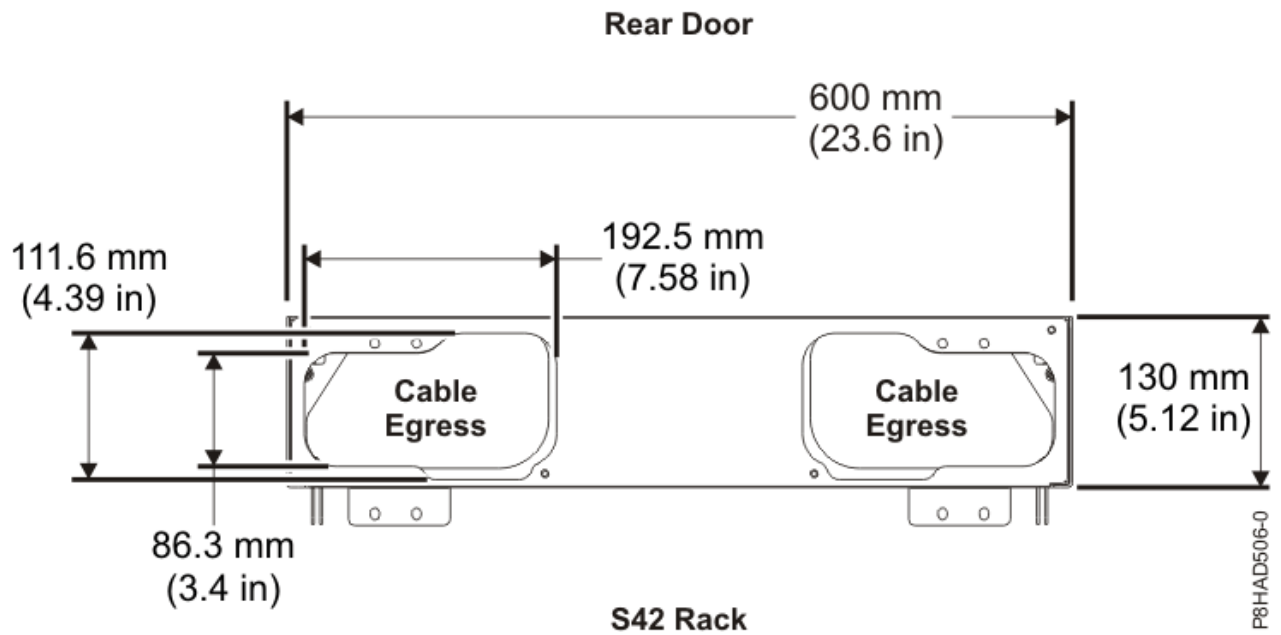
Figure 19. FC ECRK rear rack extender (top cable exit)
