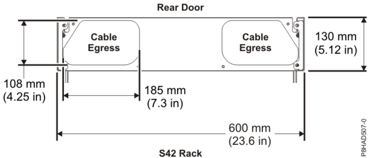
Figure 20. FC ECRK rear rack extender (bottom cable exit)
