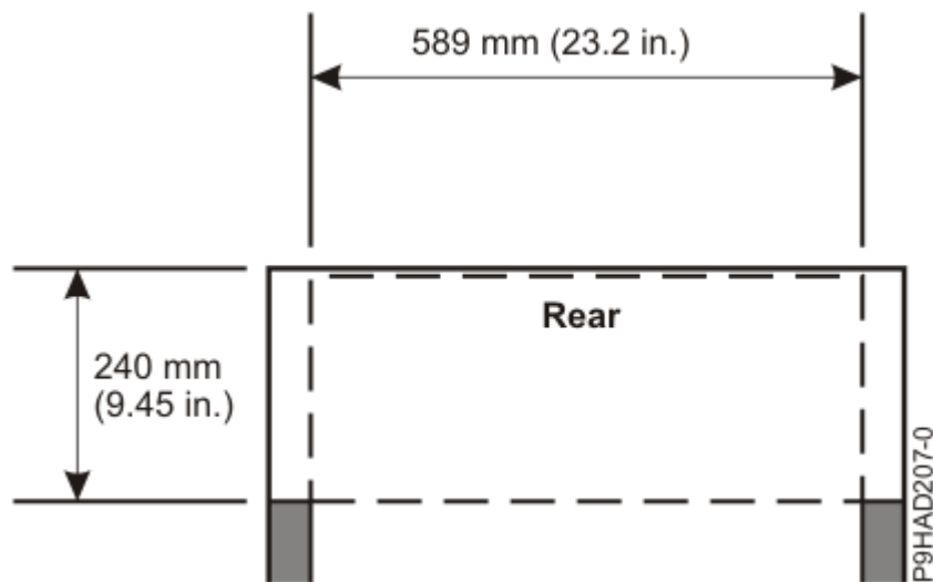
Figure 35. Model 9080-HEU rear rack clearance
