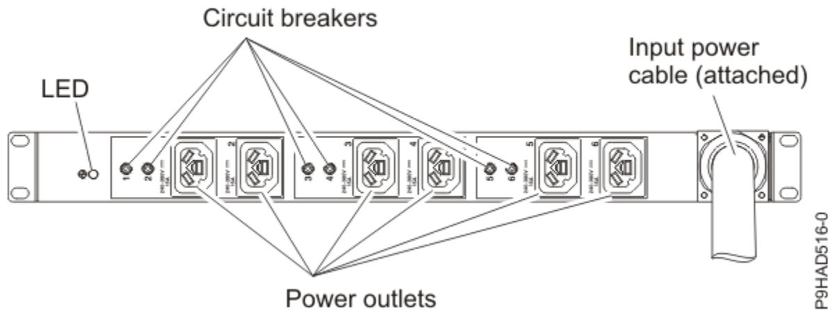
Figure 42. HVDC PDU
