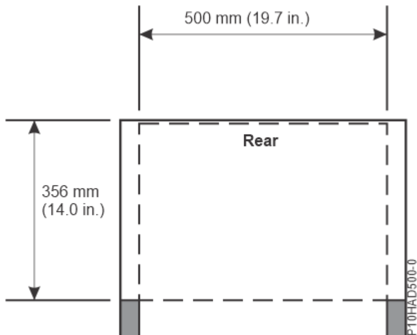
Figure 36. Model 9080-HEU rear rack clearance (narrow rack bracket installation)
