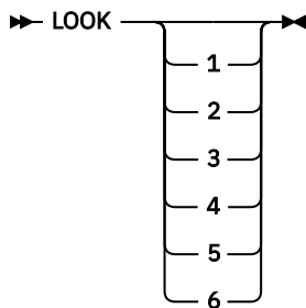
Figure 27. Syntax of the LOOK command
