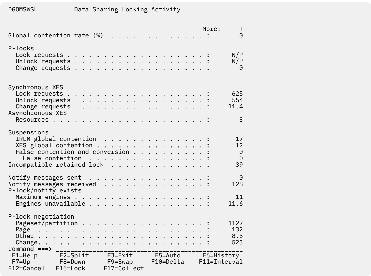
Figure 106. Data Sharing Locking Activity window
