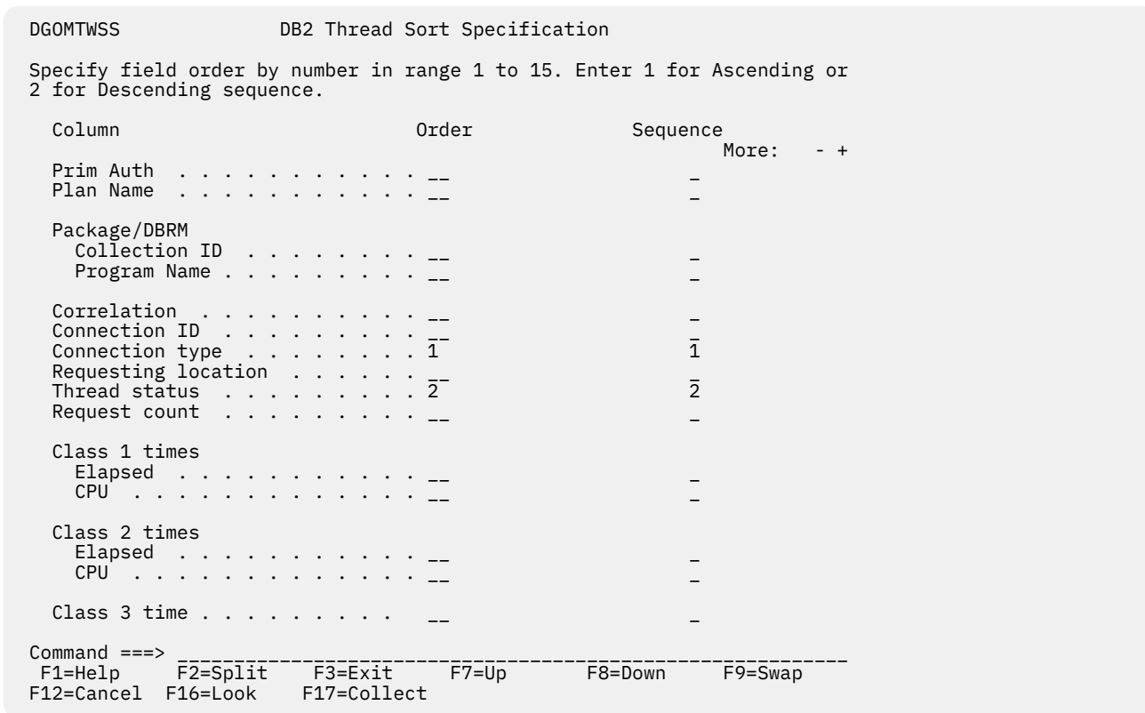
Figure 77. Db2 Thread Sort Specification window
