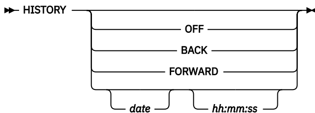
Figure 67. Syntax of the HISTORY command
