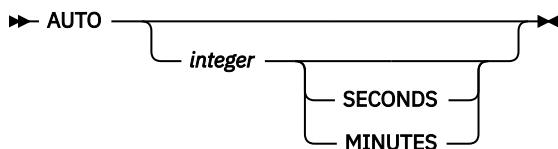
Figure 65. Syntax of the AUTO command
