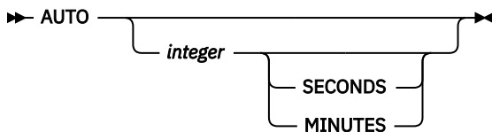
Figure 112. Syntax of the AUTO command
