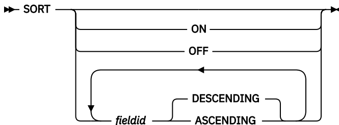
Figure 75. Syntax of the SORT command
