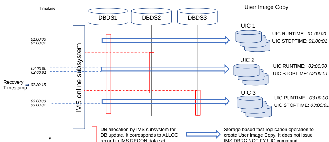
Figure 206: Creating User Image Copy using storage-based fast-replication facilities
