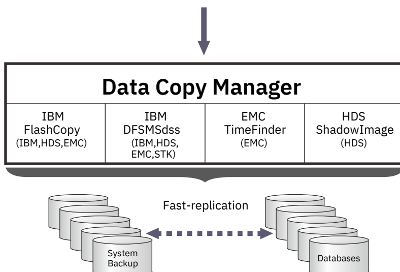
Figure 8: IMS Recovery Expert Data Copy Manager interaction with copy blades
