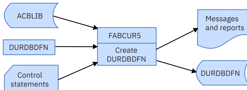
Figure 12. Flow of Database Definition Record Create utility
