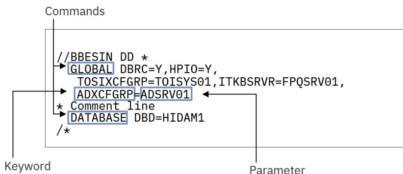
Figure 3: Format of the BBESIN control statement
