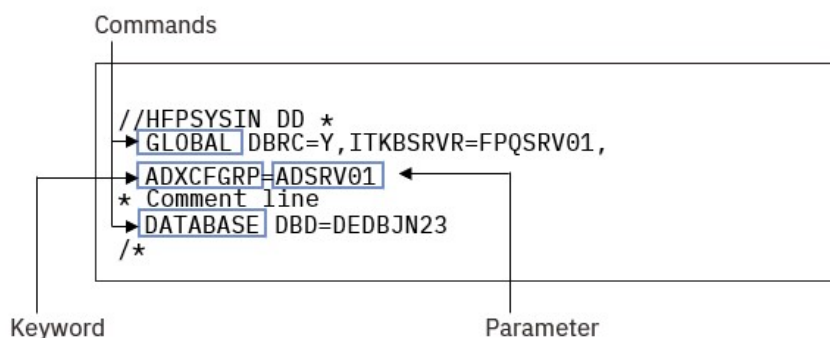
Figure 25: Format of the HFPSYSIN control statement
