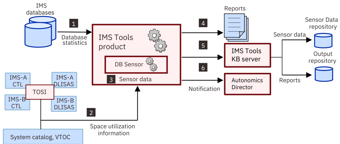
Figure 2: Integrated DB Sensor process flow
