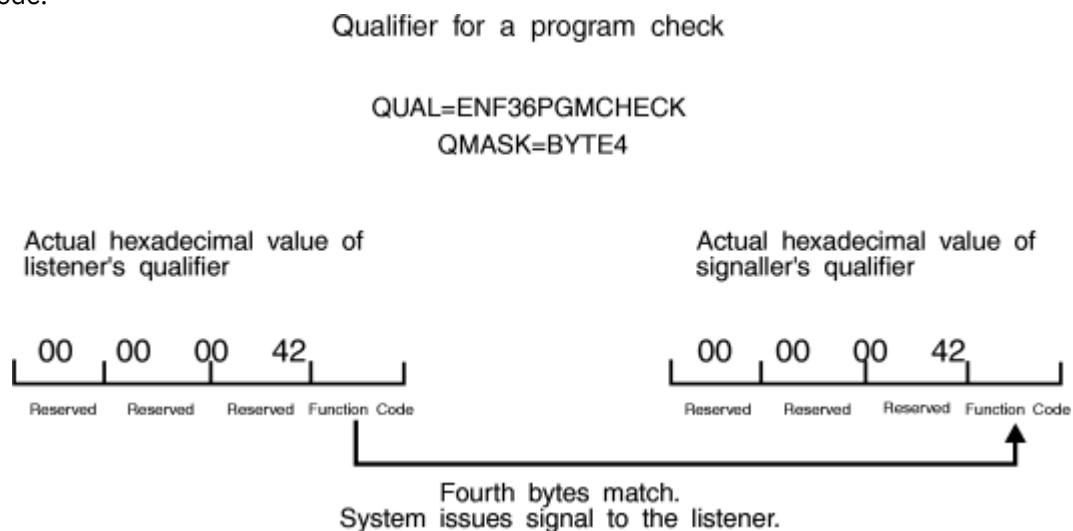
Figure 31. Qualifier for a Program Check
