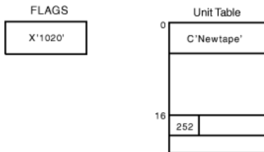
Figure 119. Input for Function Codes 3 and 10
