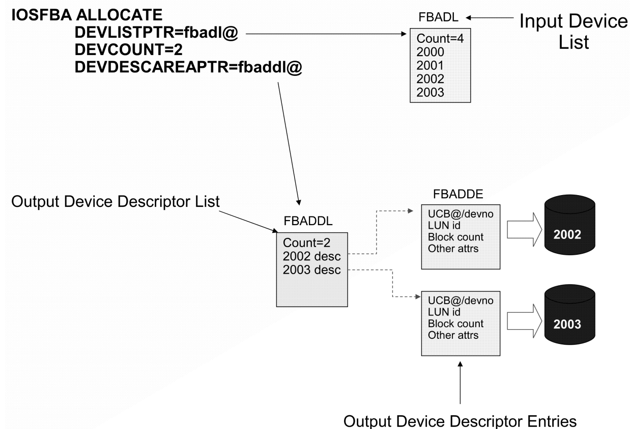
Figure 89. Visual representation of IOSFBA allocation
