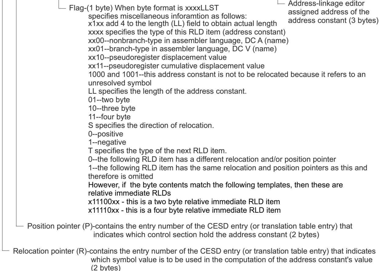
Figure 16. Relocation dictionary record (load module)
