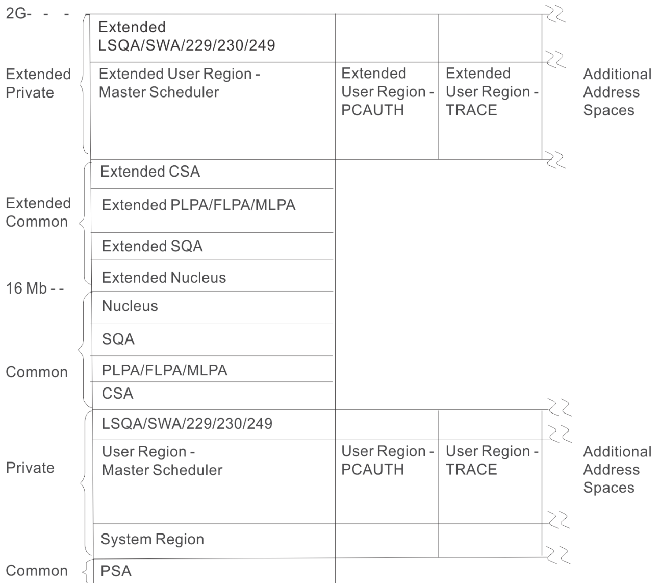
Figure 1. Virtual storage layout for multiple address spaces
