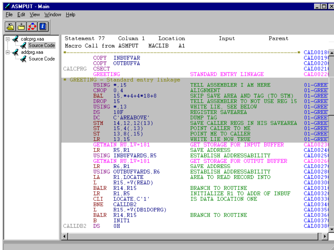
Figure 12. A source code listing displaying a set of expanded lines
