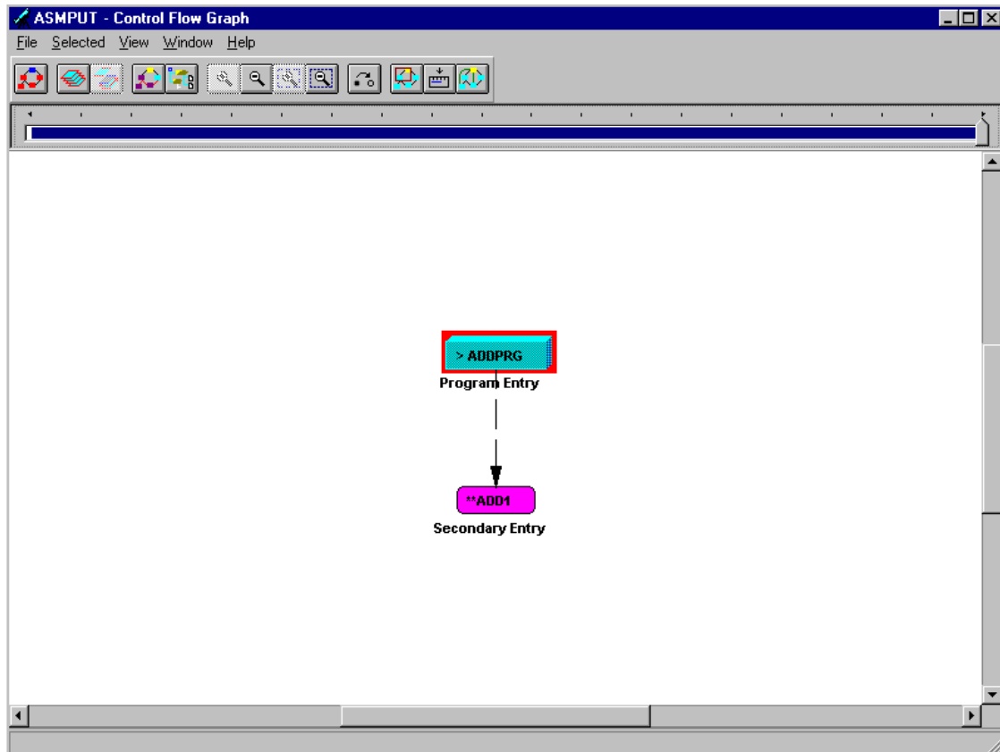
Figure 20. The same node collapsed to context
