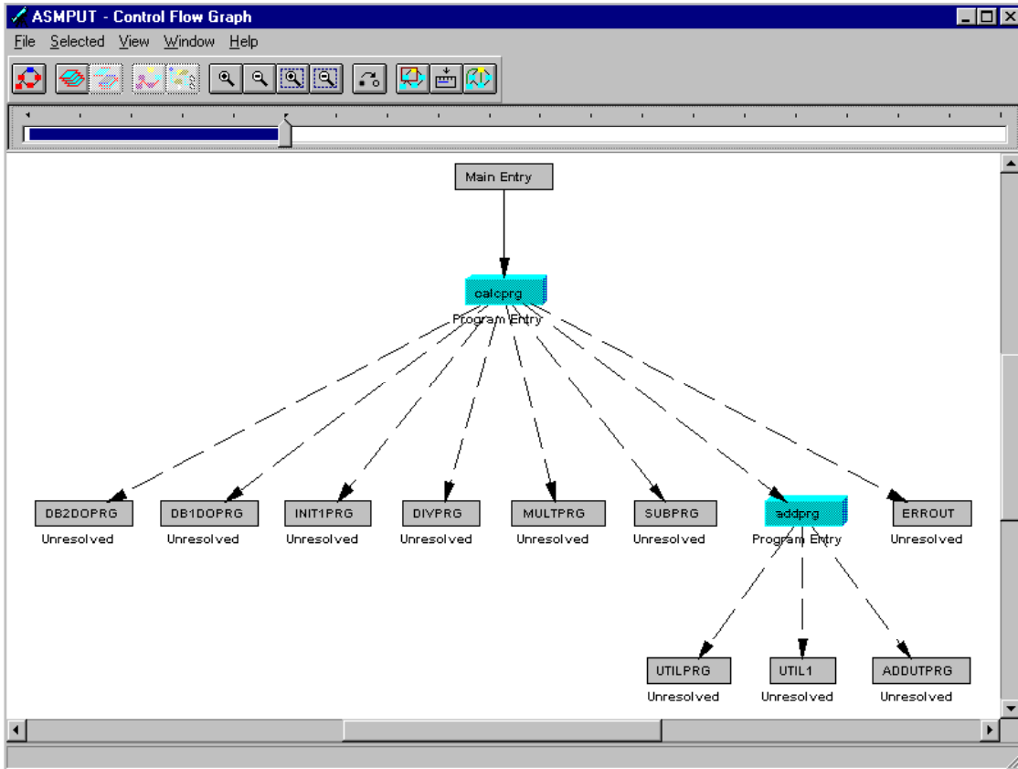
Figure 15. A completely collapsed control flow graph
