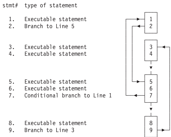
Figure 8. An example of code and nodes
