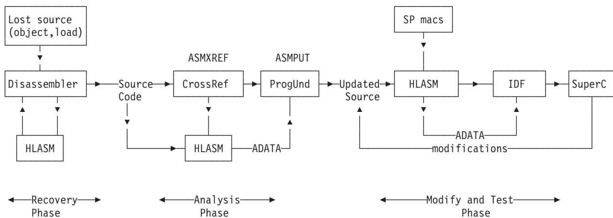
Figure 5. Toolkit Feature: Summary of Usage Phases
