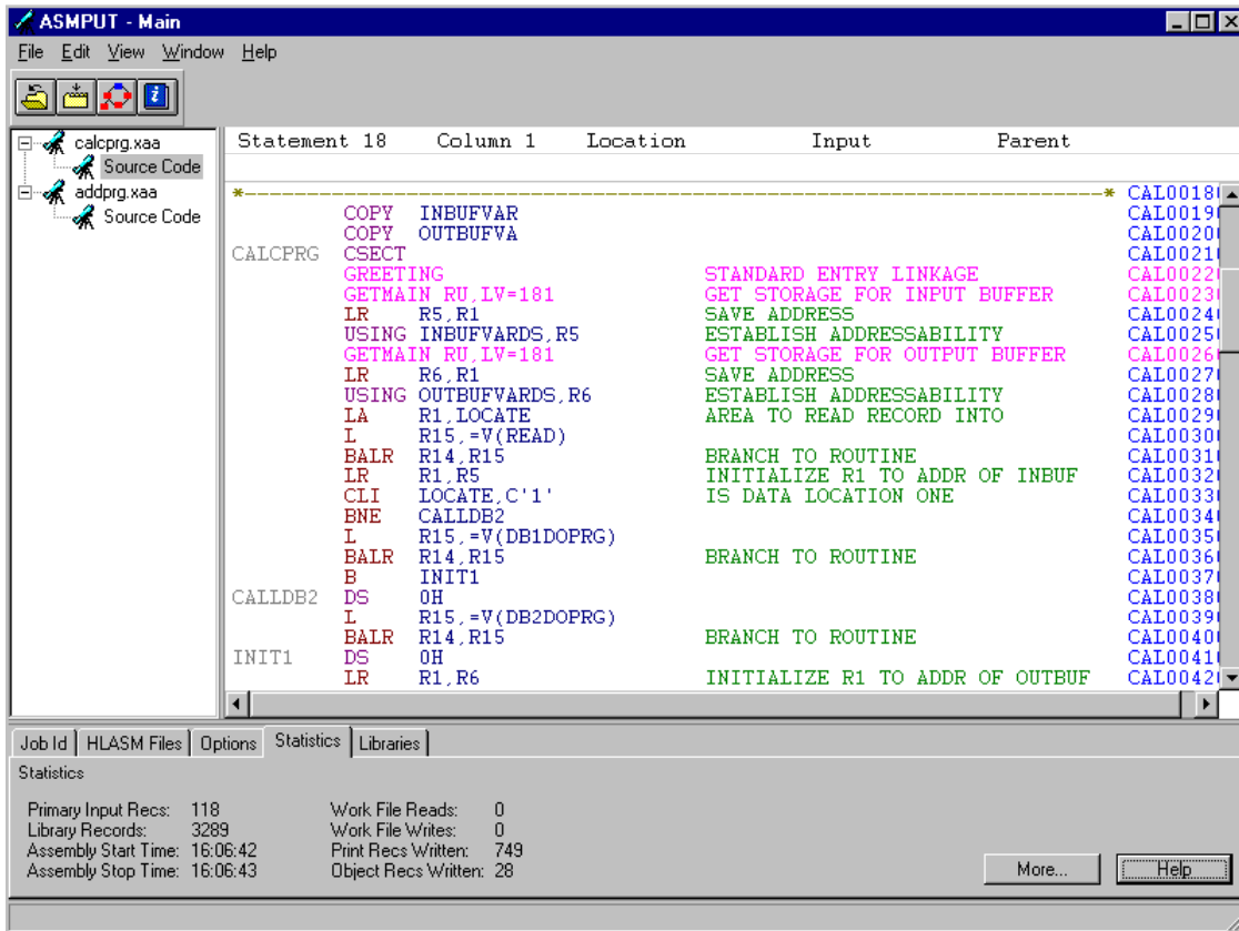
Figure 13. The information notebook Statistics tab
