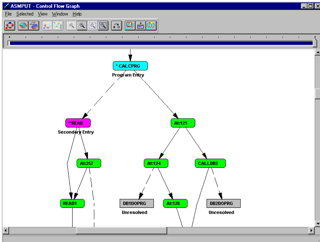
Figure 24. A graph at maximum zoom
