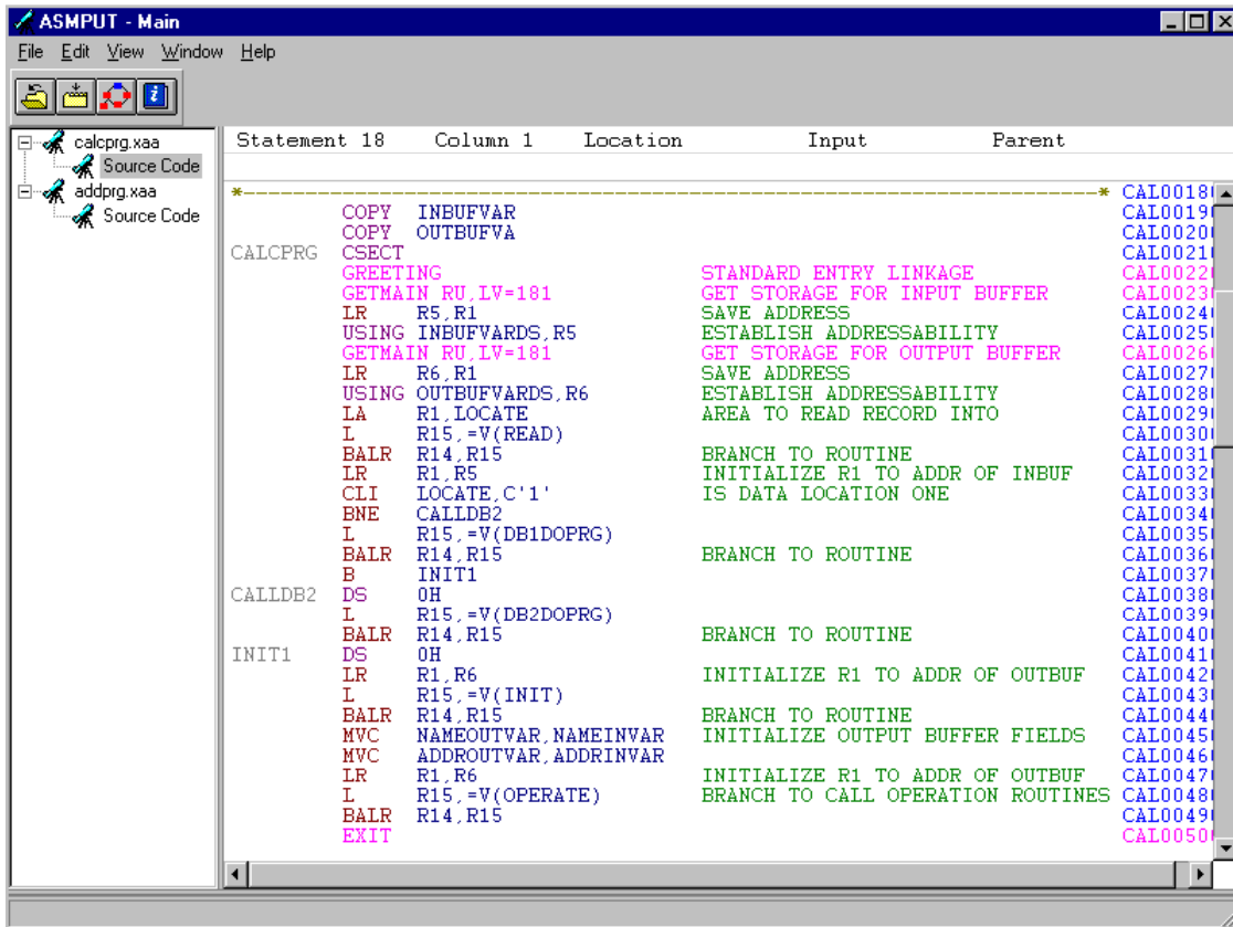
Figure 11. A source code listing not displaying any expanded lines
