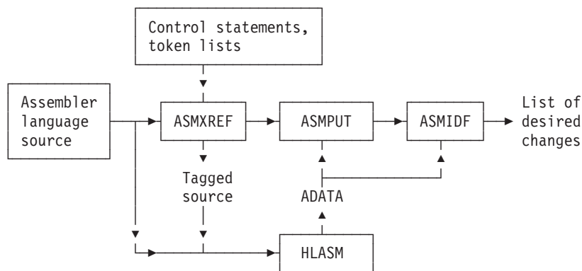
Figure 3. Toolkit Feature: Analysis and Understanding Phase
