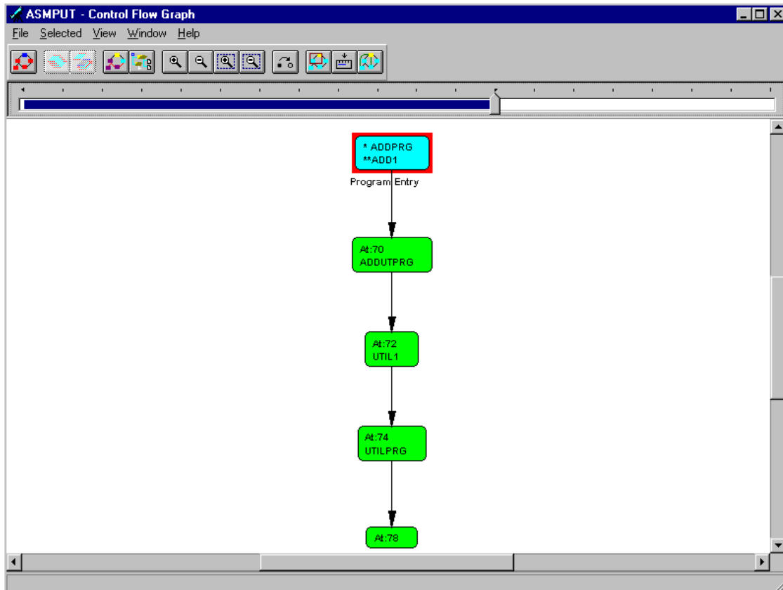
Figure 19. One node expanded to the window
