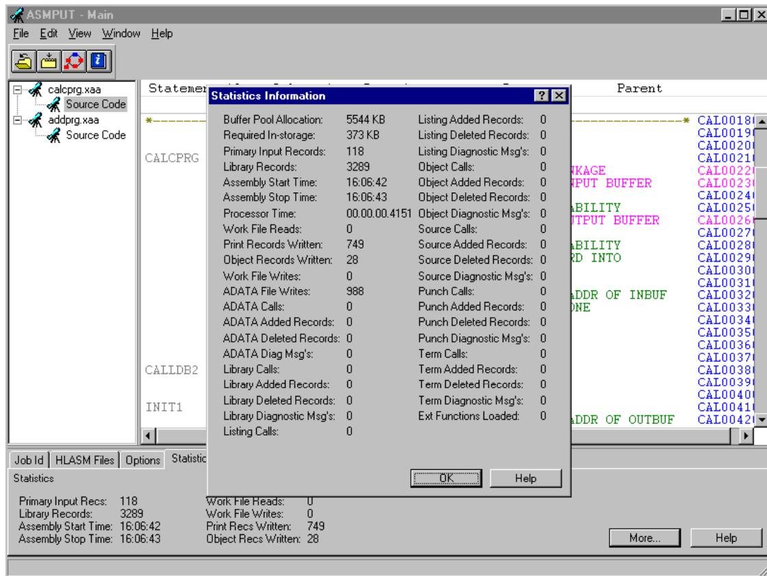
Figure 14. More Statistics information
