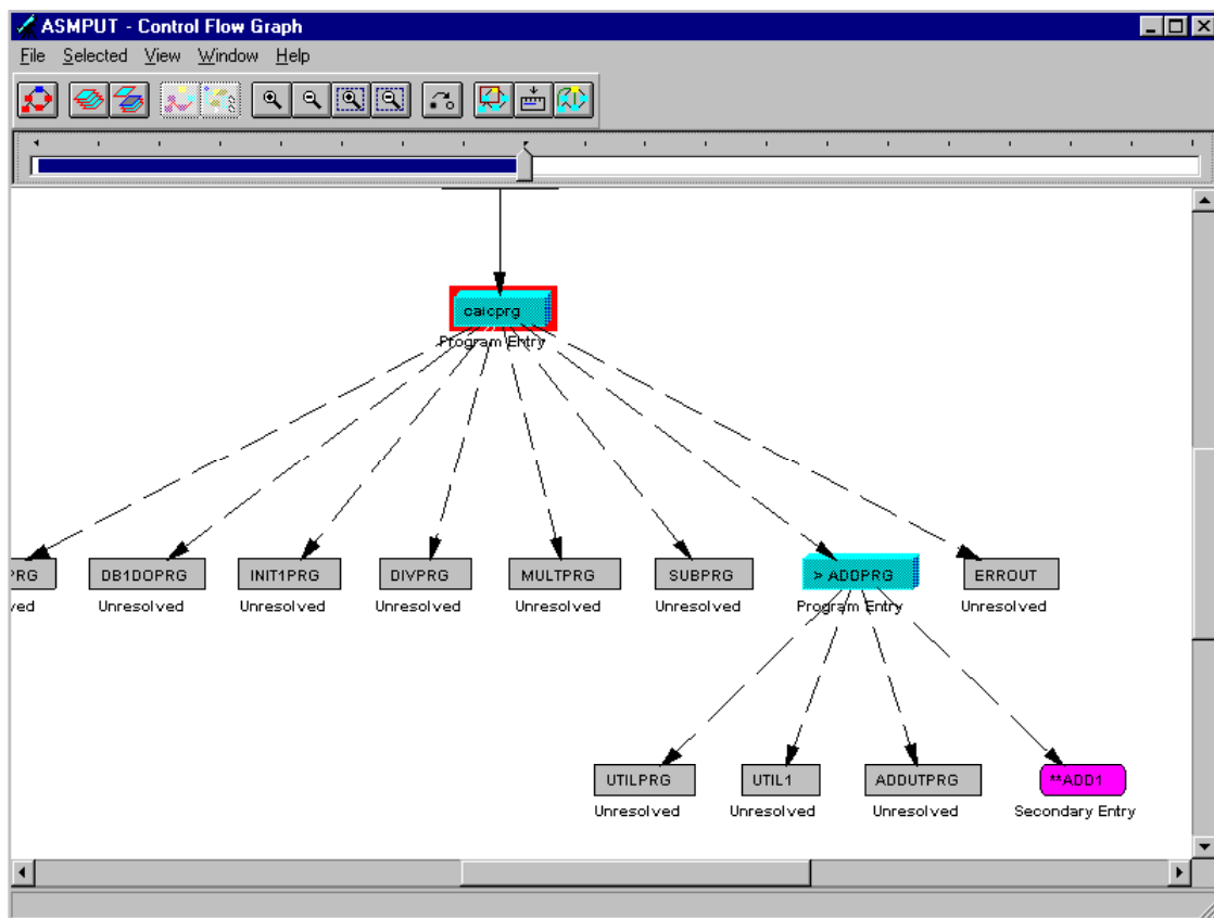
Figure 18. One node expanded in context
