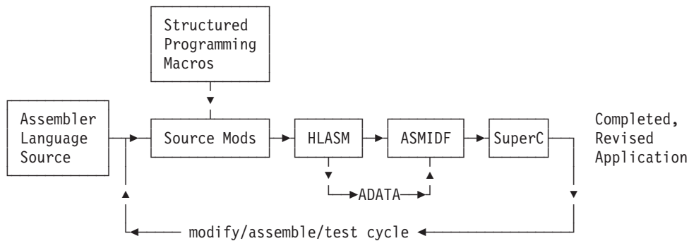
Figure 4. Toolkit Feature: Modification and Testing Phase
