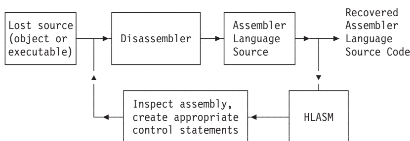
Figure 2. Toolkit Feature: Recovery and Reconstruction Phase
