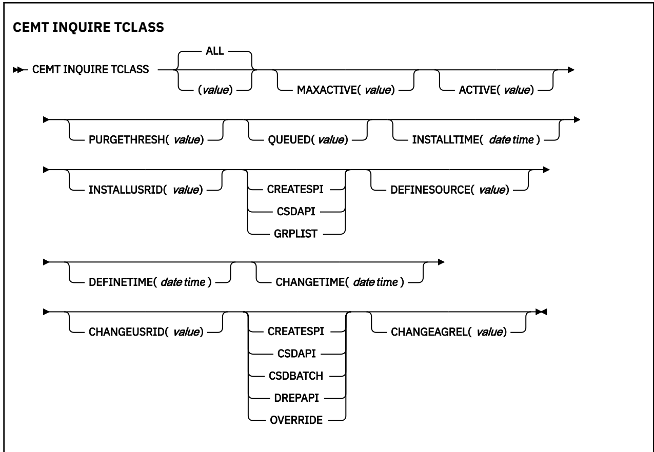
Figure 81. The expanded display of an individual entry
