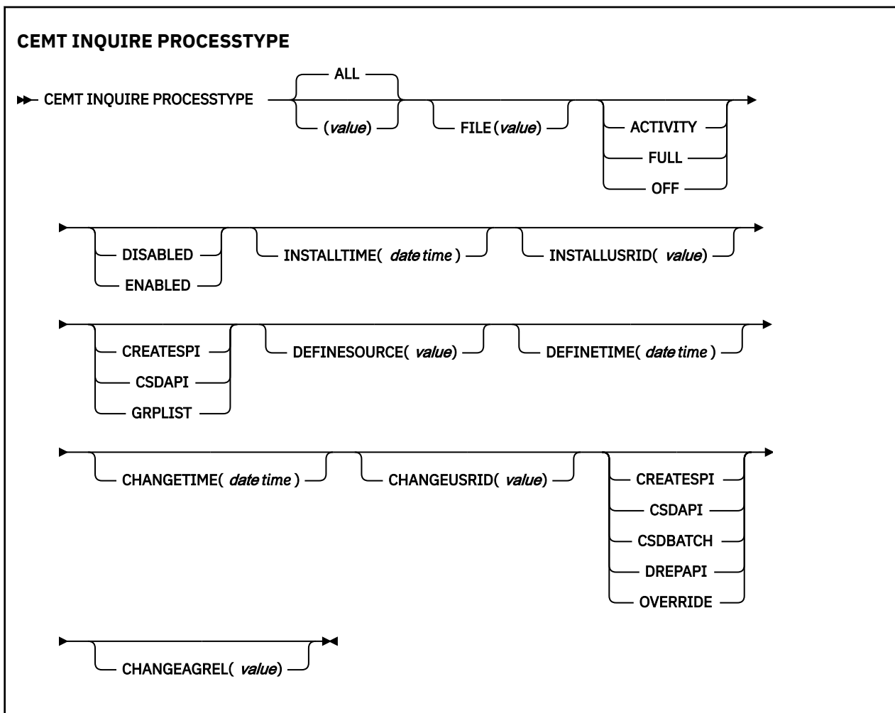
Figure 69. The expanded display of an individual entry
