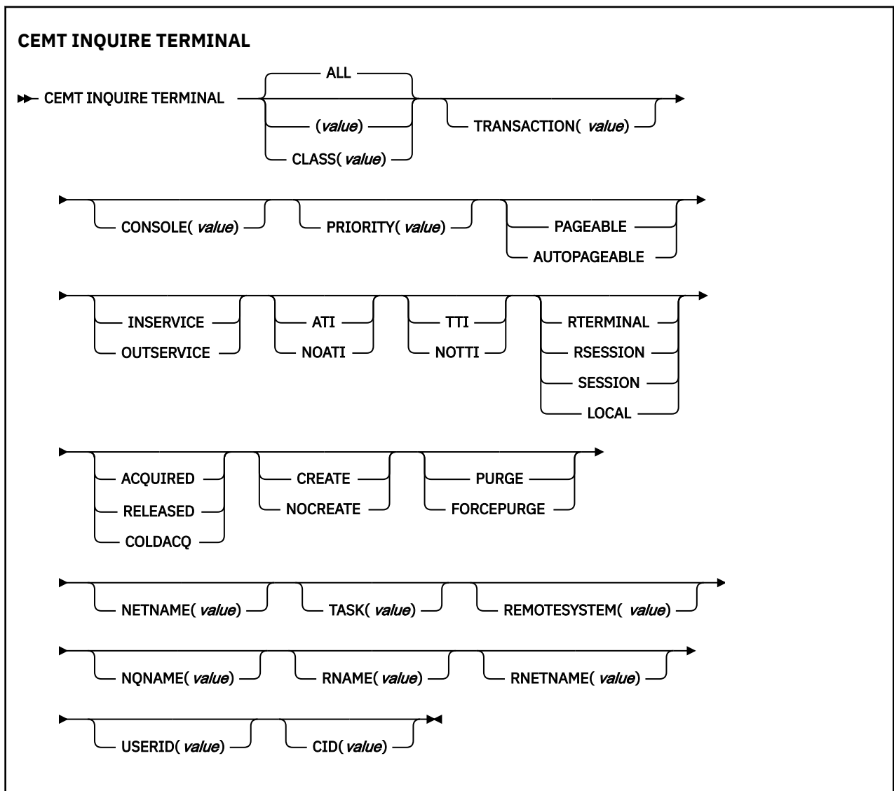
Figure 85. The expanded display of an individual entry
