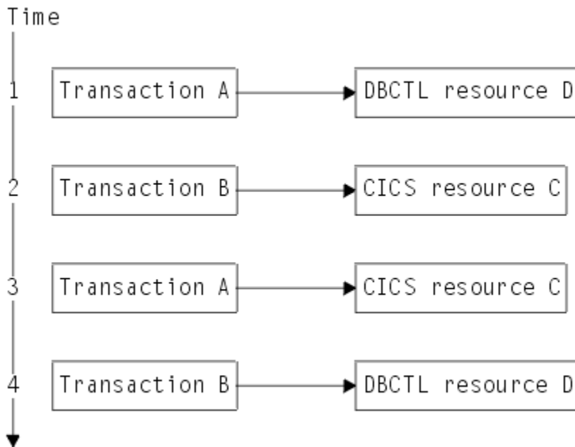
Figure 29. Transaction deadlock
