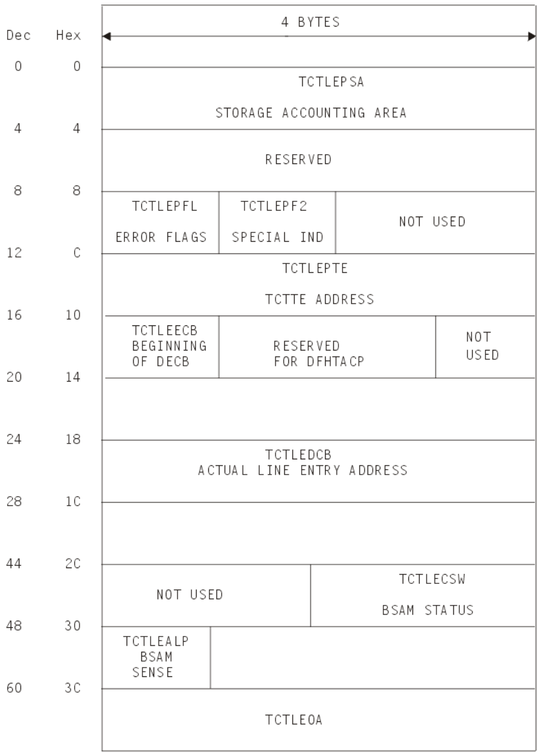
Figure 23. Graphical description of the format of the TACLE DSECT: TERMINAL ABNORMAL CONDITION LINE ENTRY
