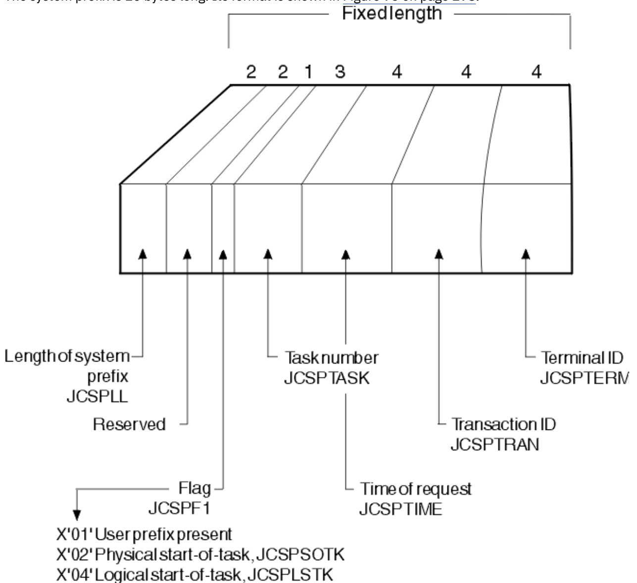
Figure 90. Format of the system prefix
