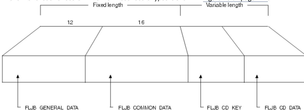
Figure 70. Layout of record written for read-only, read-update, write-update, write-add, and write-add-complete record types
