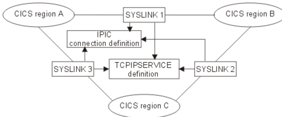
Figure 10. An example of reusing definitions to create connections
