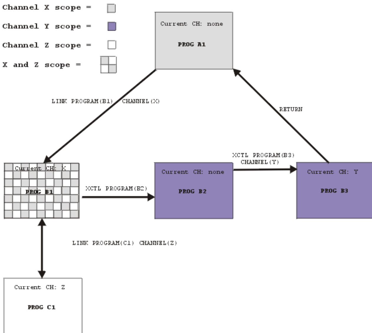
Figure 39. The scope of a channel—example showing LINK and XCTL commands
