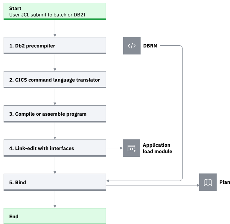
Figure 182. Steps to prepare a CICS application program that accesses Db2
