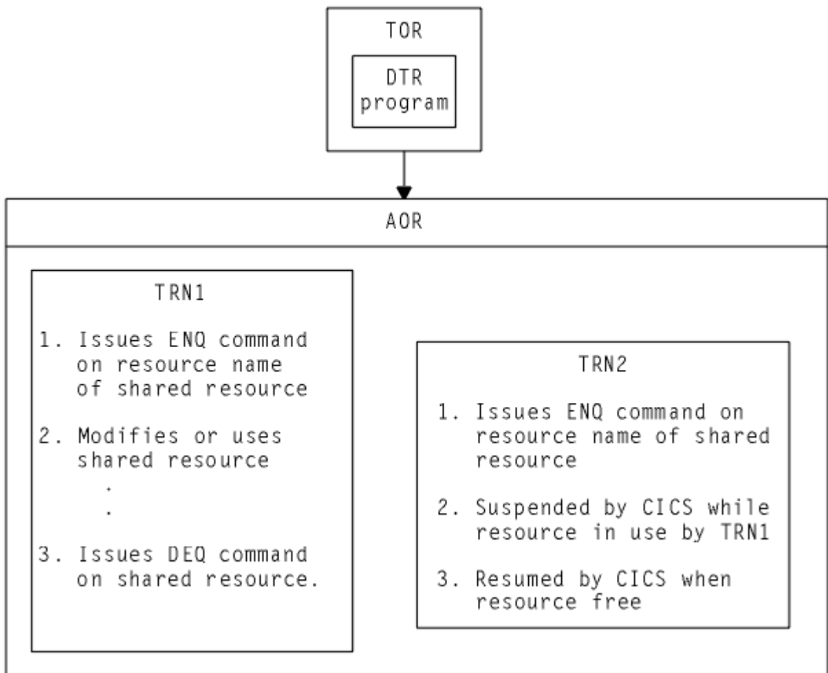
Figure 60. Illustration of inter-transaction affinity created by use of ENQ/DEQ commands
