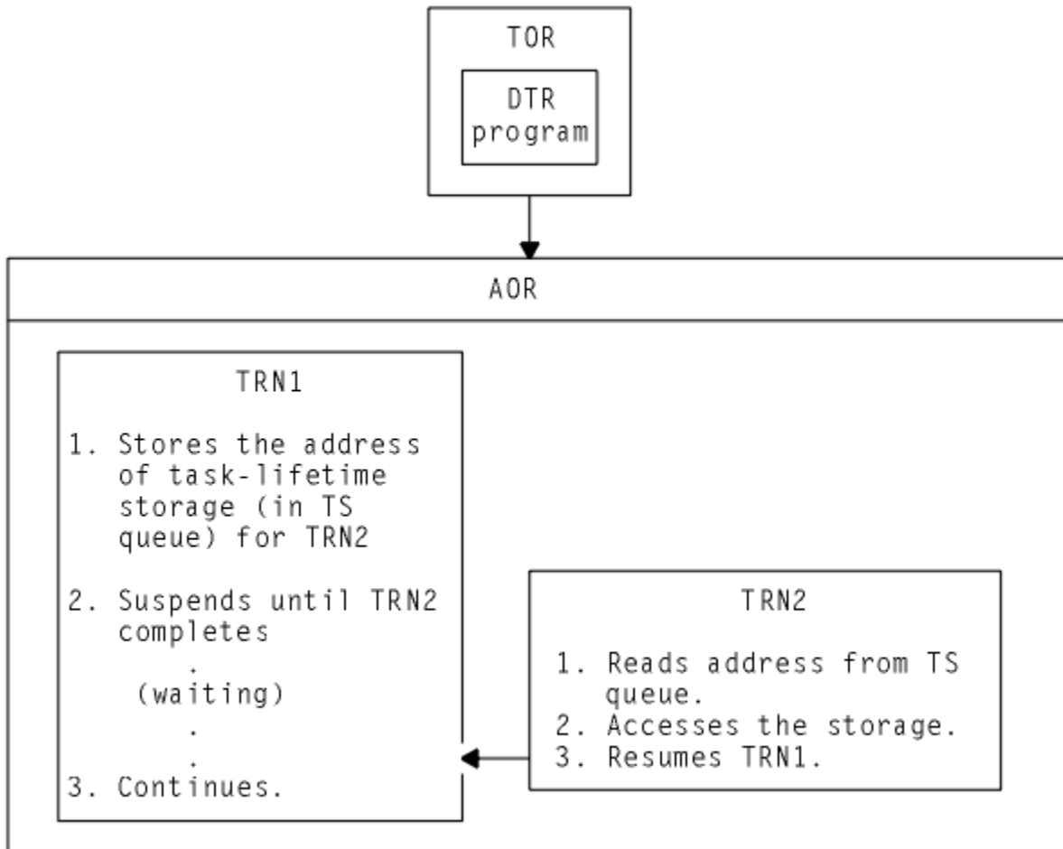
Figure 58. Illustration of inter-transaction affinity created by use of task-lifetime storage
