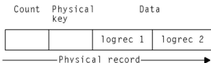
Figure 84. Blocked-data set
