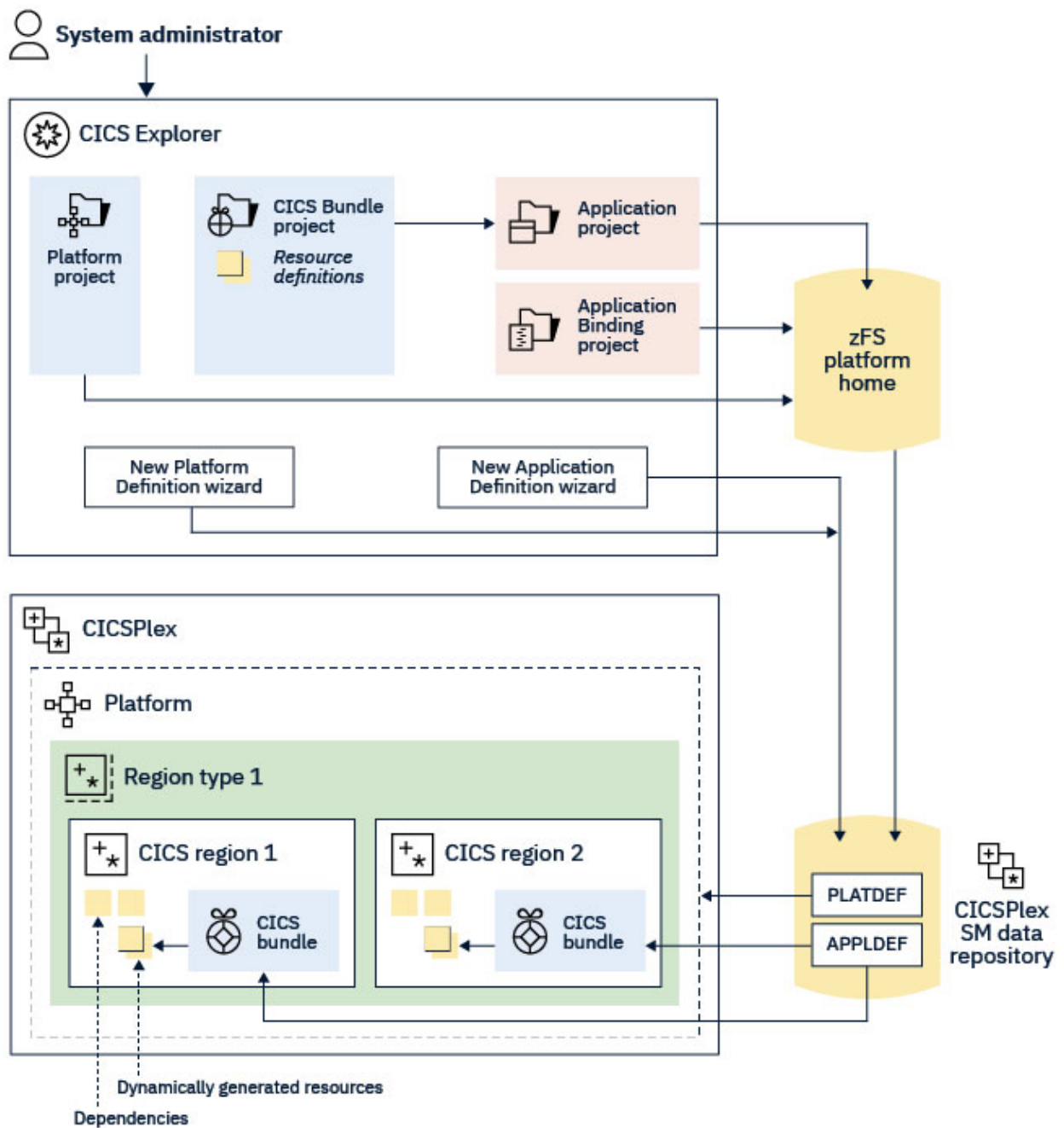
Figure 8. Cloud topology
