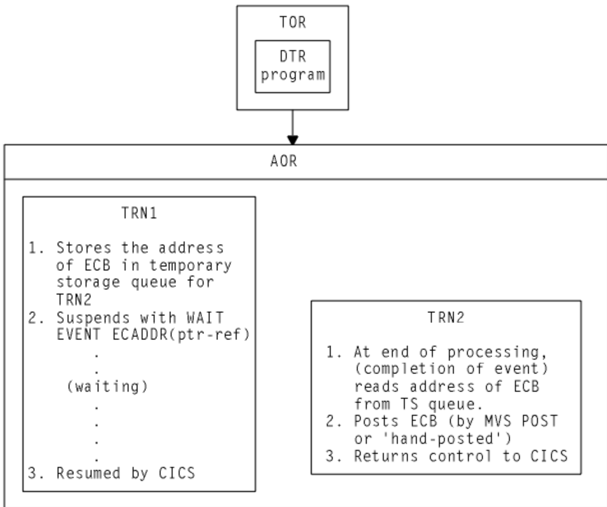
Figure 59. Illustration of inter-transaction affinity created by use of WAIT EXTERNAL command
