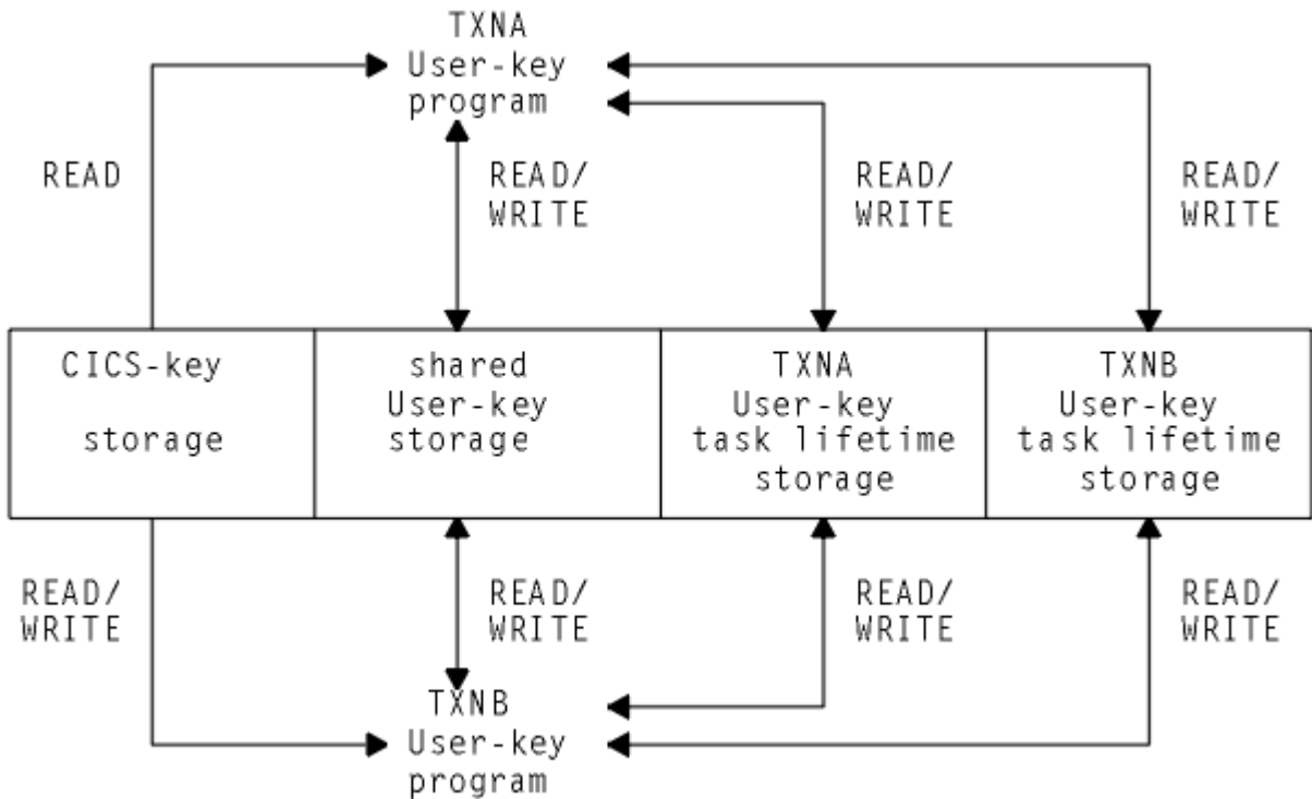
Figure 98. Two transactions defined as ISOLATE(NO) with read/write access to each other's task lifetime storage
