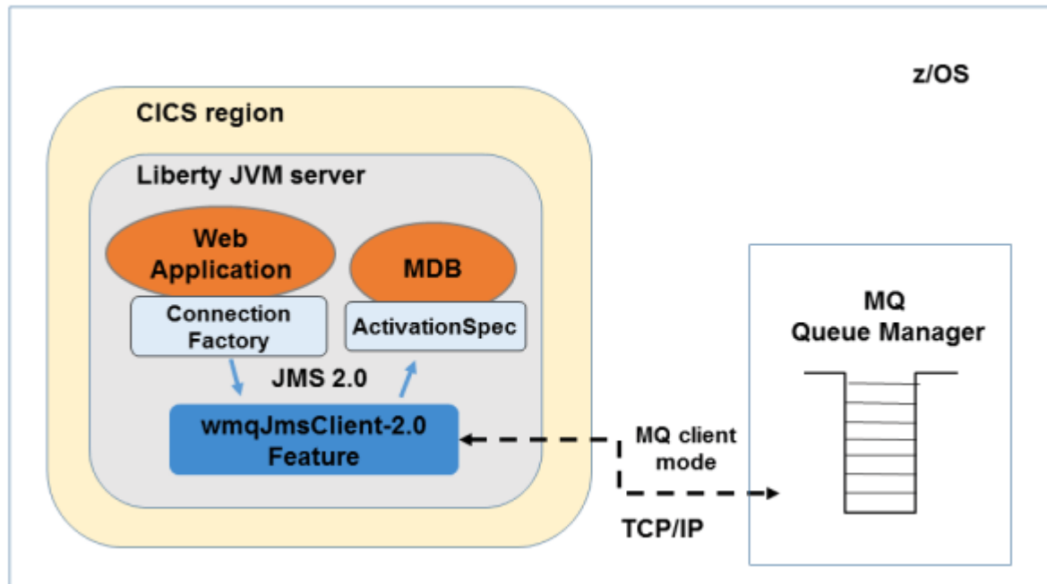
Figure 12. Applications connecting to IBM MQ using JMS and running in a CICS OSGi server
