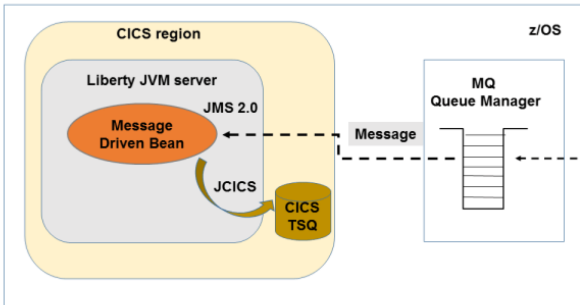
Figure 11. Accessing IBM MQ through a Java application that uses MDBs
