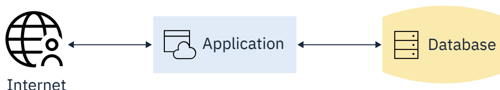
Figure 4. Monolithic architecture
