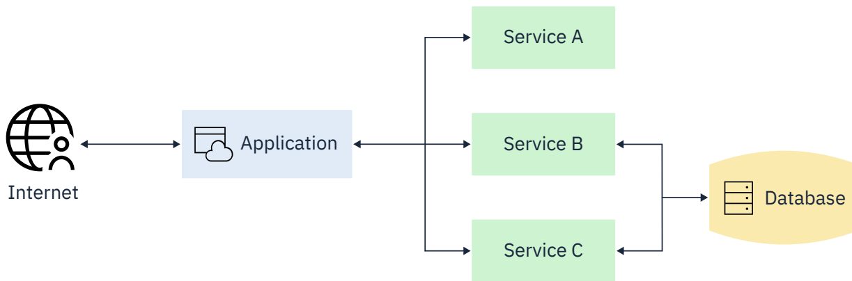
Figure 6. Hosted services
