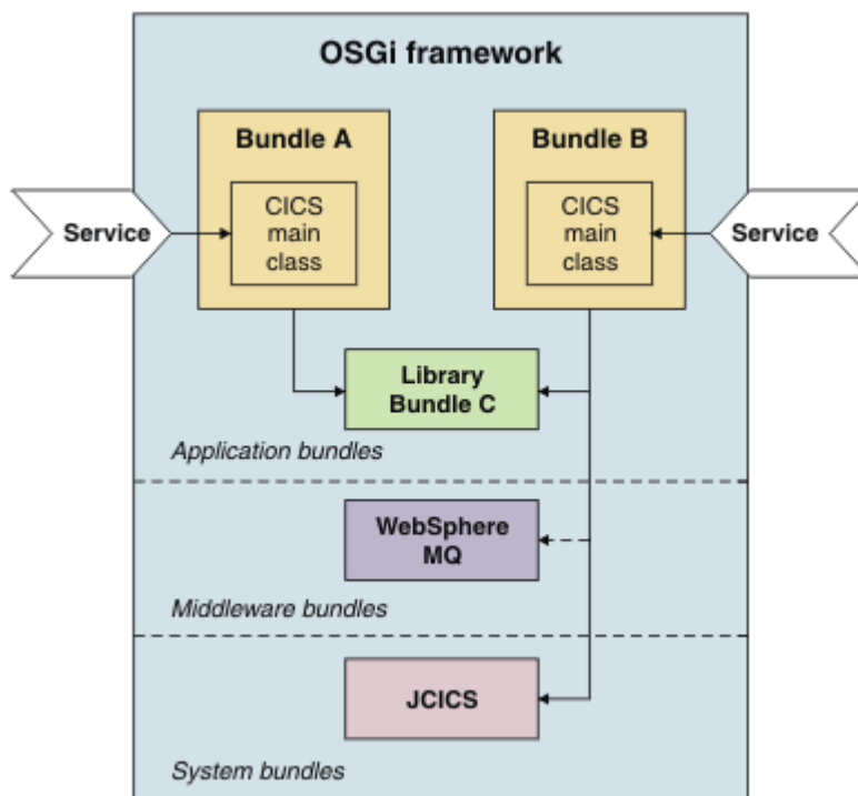
Figure 13. OSGi framework
