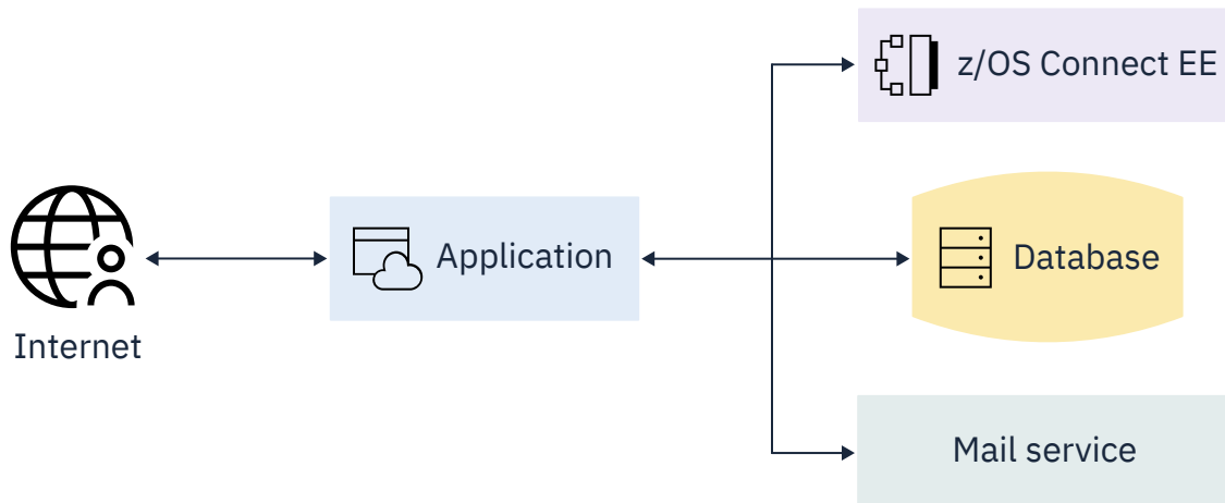
Figure 5. Backing services
