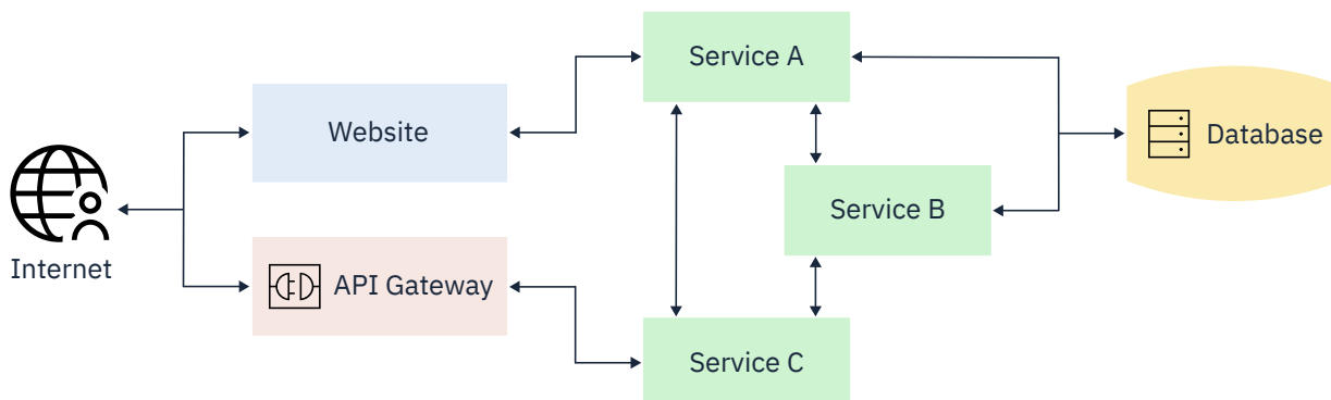
Figure 7. Microservices
