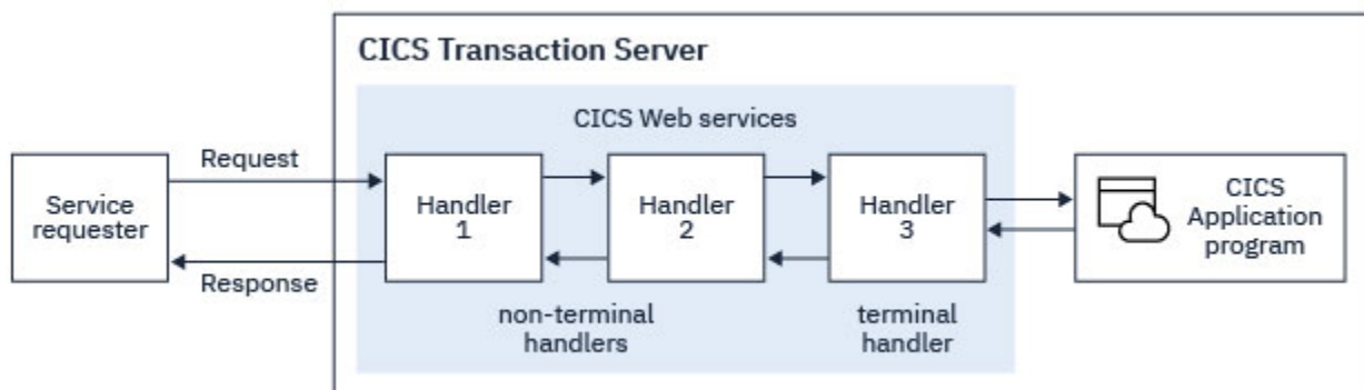
Figure 4. A service provider pipeline
