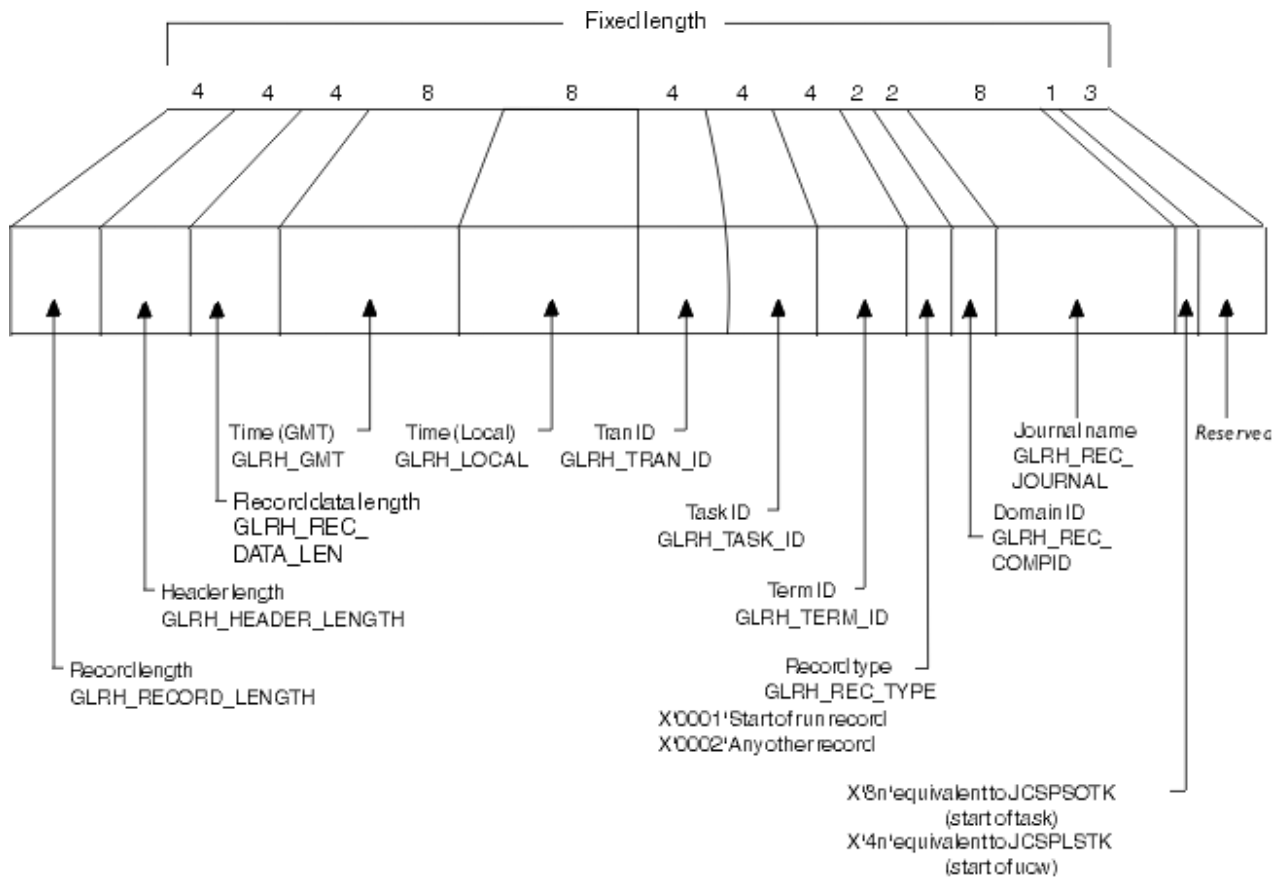
Figure 68. Format of a general log record header
