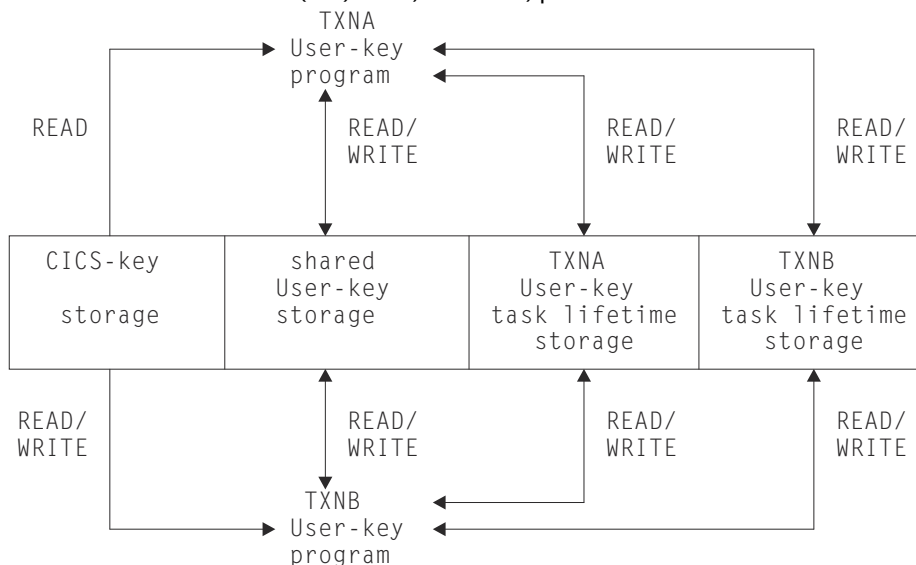
Figure 75. Two transactions defined as ISOLATE(NO) with read/write access to each other's task lifetime storage
