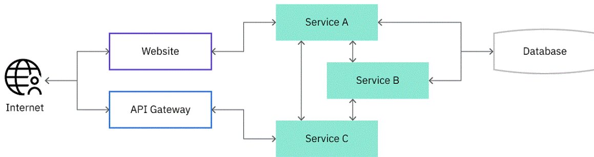
Figure 118. Microservices
