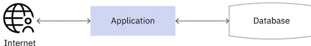
Figure 115. Monolithic architecture
