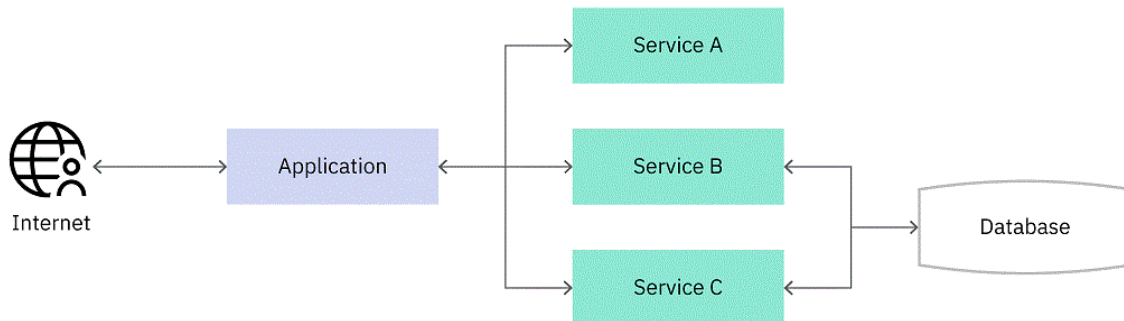
Figure 117. Hosted services
