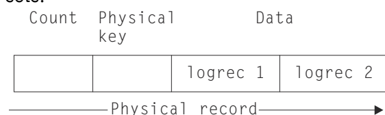
Figure 61. Blocked-data set
