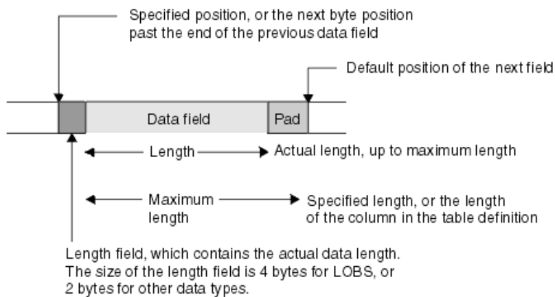
Figure 15. Layout of a varying-length field (NOT NULL) without the NOPAD option
