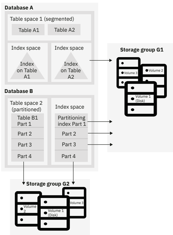
Figure 13. Hierarchy of Db2 structures
