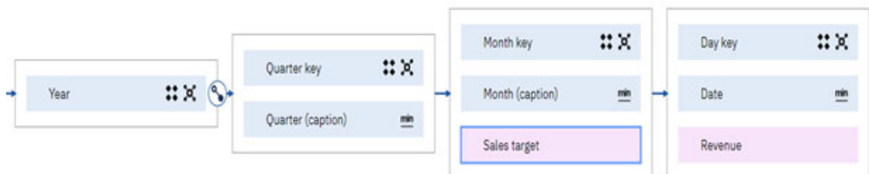
Figure 9. Example of column dependencies for scenario 1
