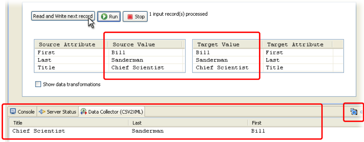
Figure 94. One record read and collected
