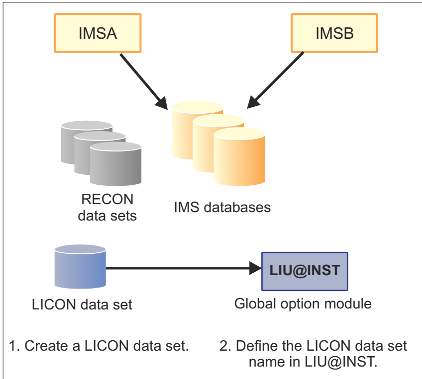
Figure 2. Integrity Checker configuration in a data-sharing environment
