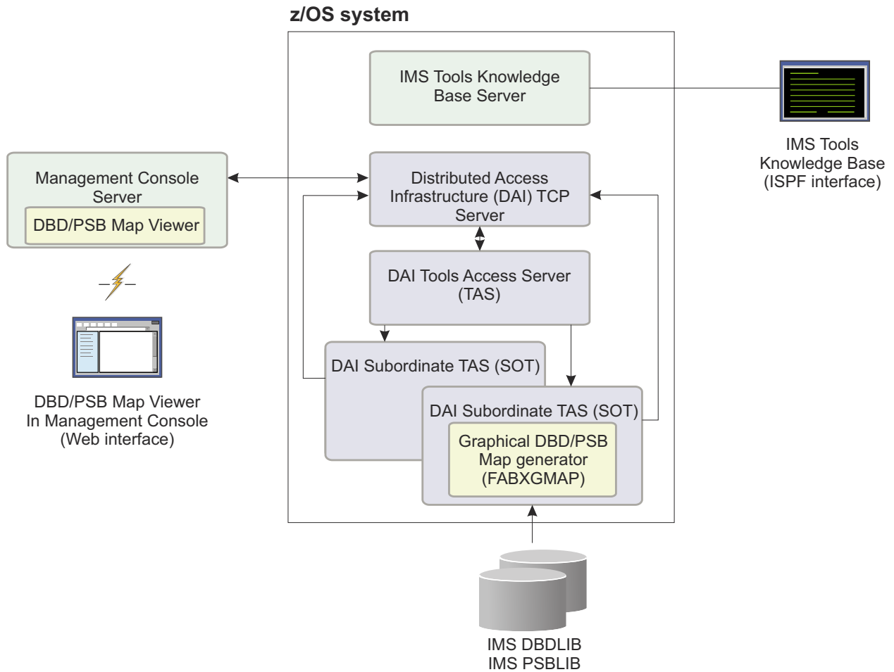
Figure 10. DBD/PSB Map Viewer configuration
