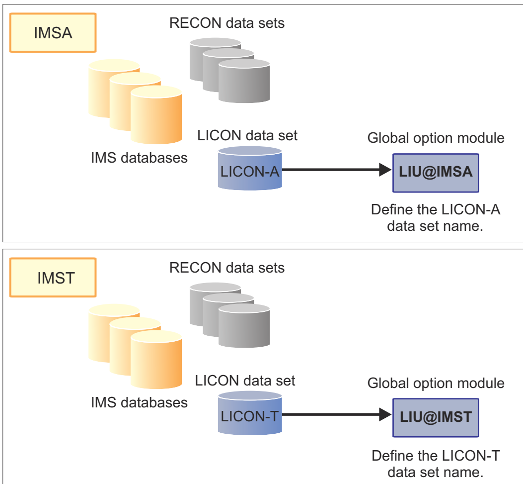
Figure 3. Integrity Checker configuration in a non-data-sharing environment
