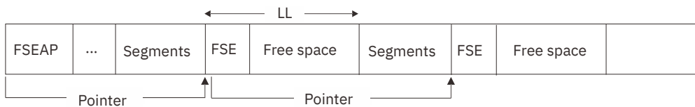
Figure 138. Structure of the free space element (FSE)
