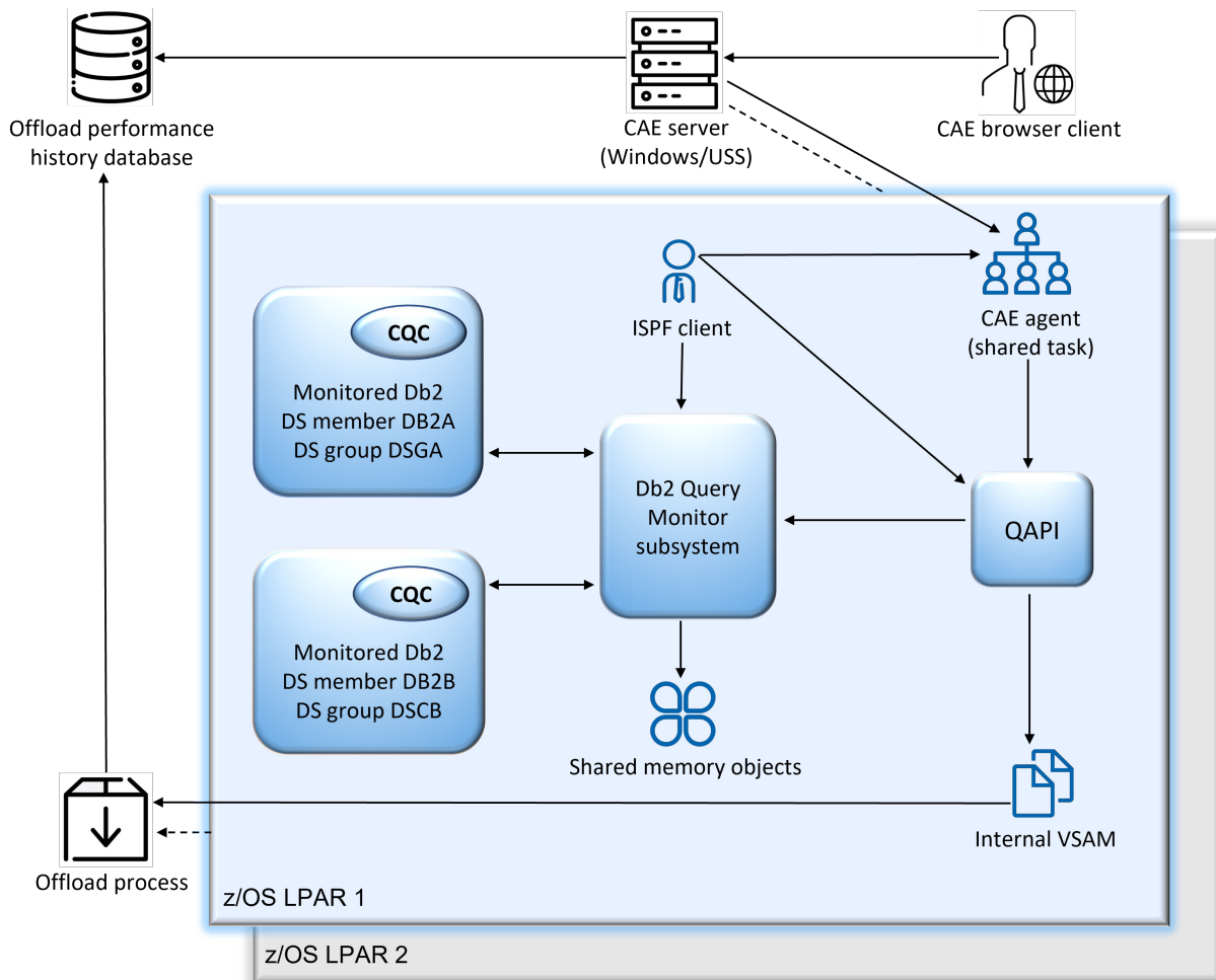
Figure 1. Db2 Query Monitor architecture
