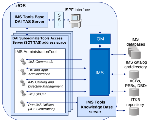
Figure 1: Server and component architecture of a single IMS Administration Tool system in a single LPAR
