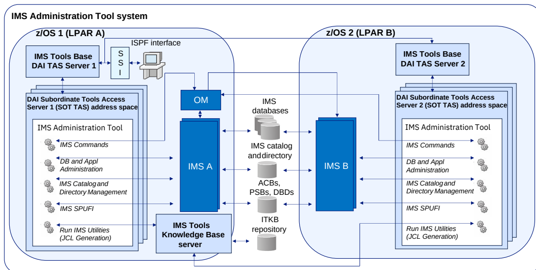
Figure 2: Server and component architecture of a single IMS Administration Tool system in a multiple-LPAR configuration
