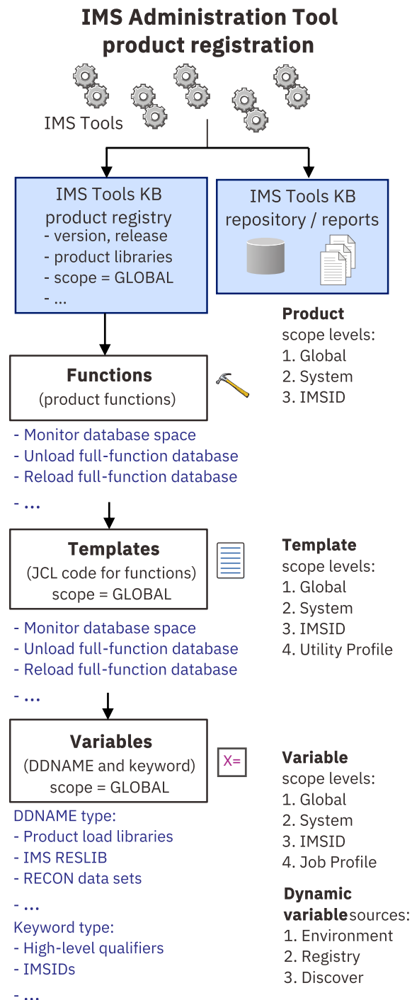
Figure 3: Product registration process flow
