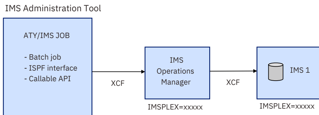
Figure 18: IMS Operations Manager (OM) configuration
