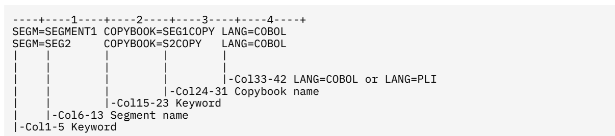
Figure 4: Type-0 copybook XREF statement syntax
