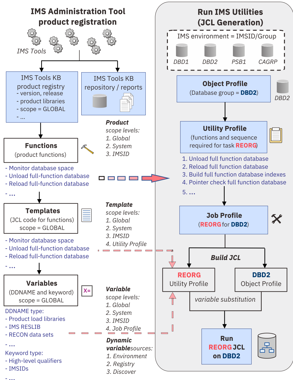
Figure 17: JCL generation process flow
