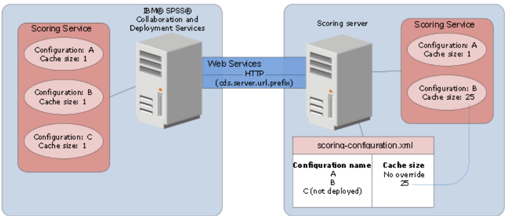
Figure 4. Scoring server environment configuration
