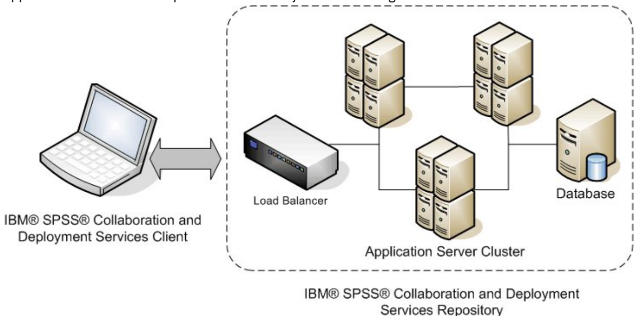
Figure 5. Cluster architecture
