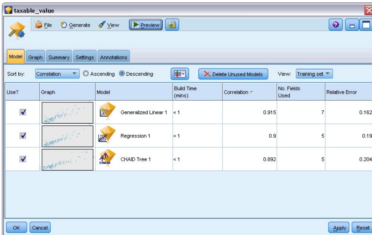
Figure 48. Auto Numeric results
