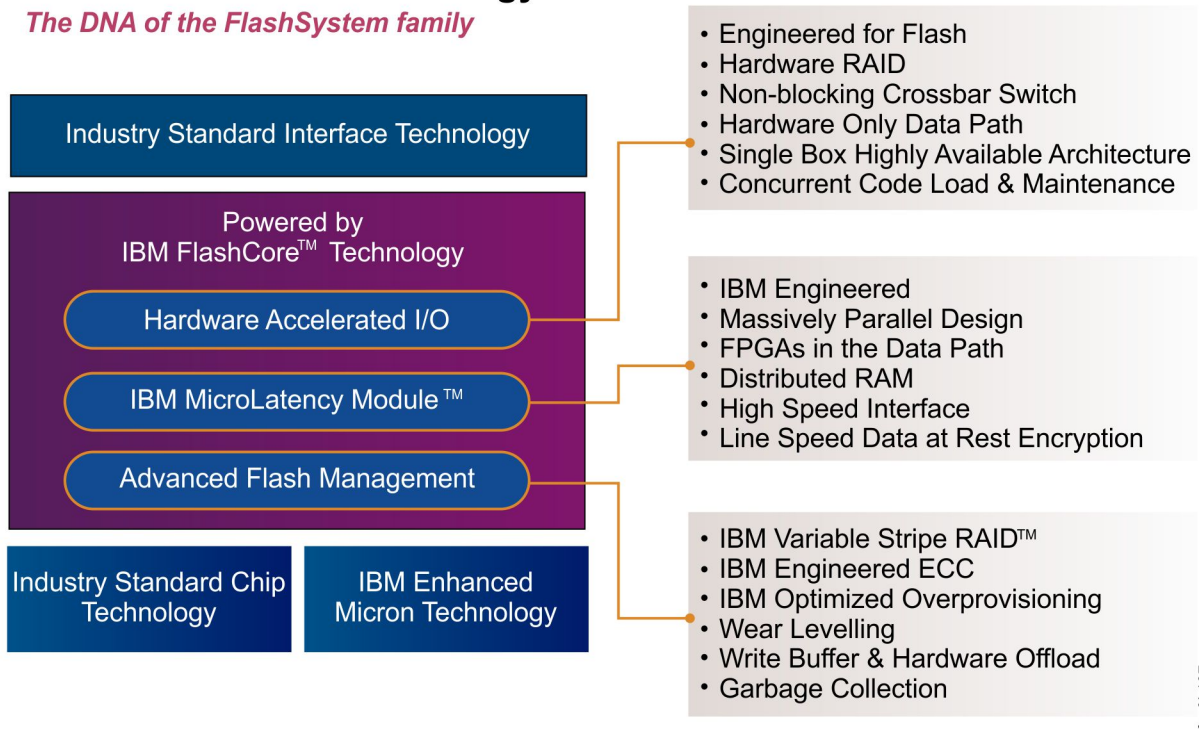
Figure 3. IBM FlashCore technology benefits
