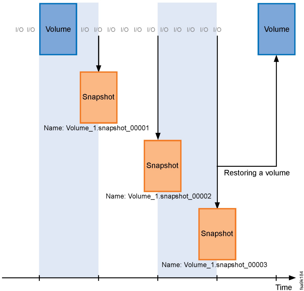
Figure 22. Restoring volumes
