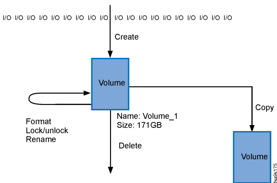
Figure 16. Volume operations
