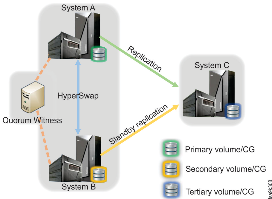
Figure 52. Multi-site HA/DR diagram
