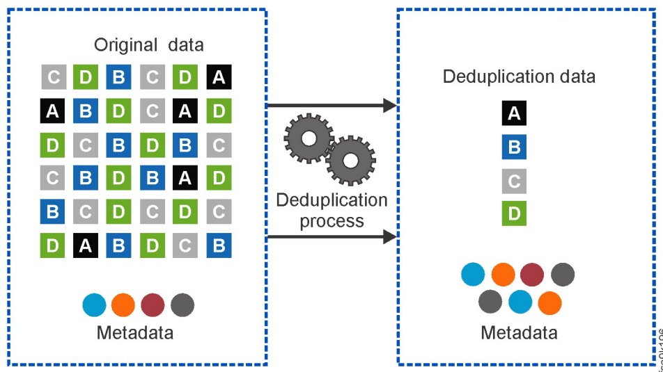
Figure 8. Deduplication process
