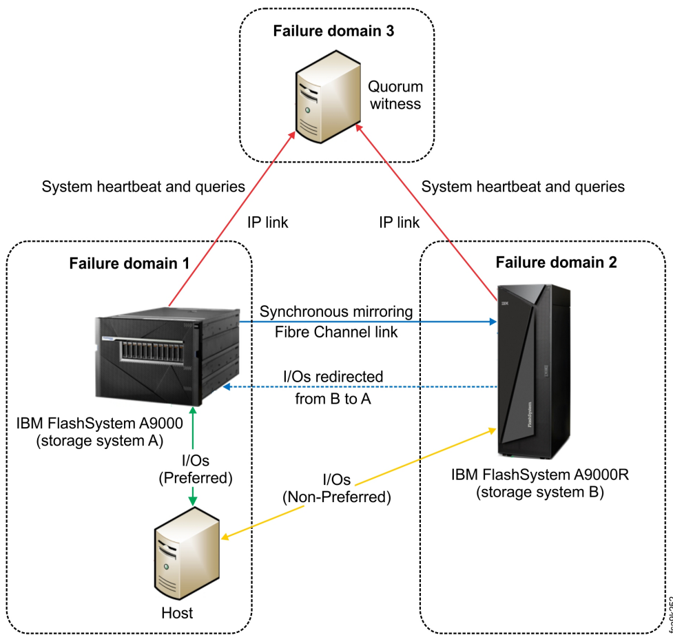
Figure 36. Typical HyperSwap high availability configuration
