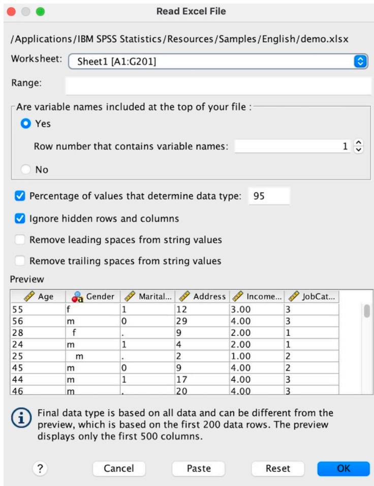
Figure 11. Read Excel File dialog
