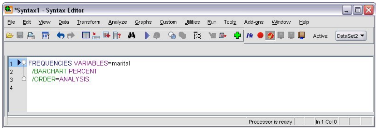
Figure 70. Frequencies syntax
