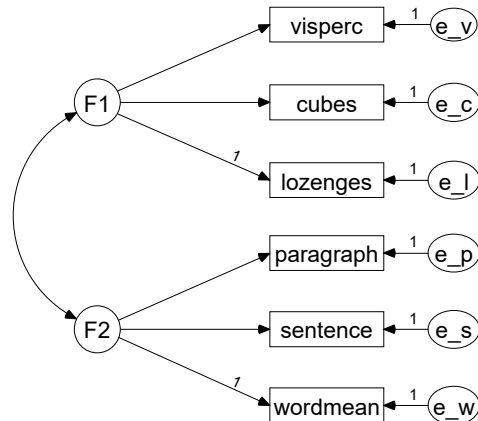
Example 20: Model 2R Restricted two-factor model Holzinger and Swineford (1939) data Model Specification
