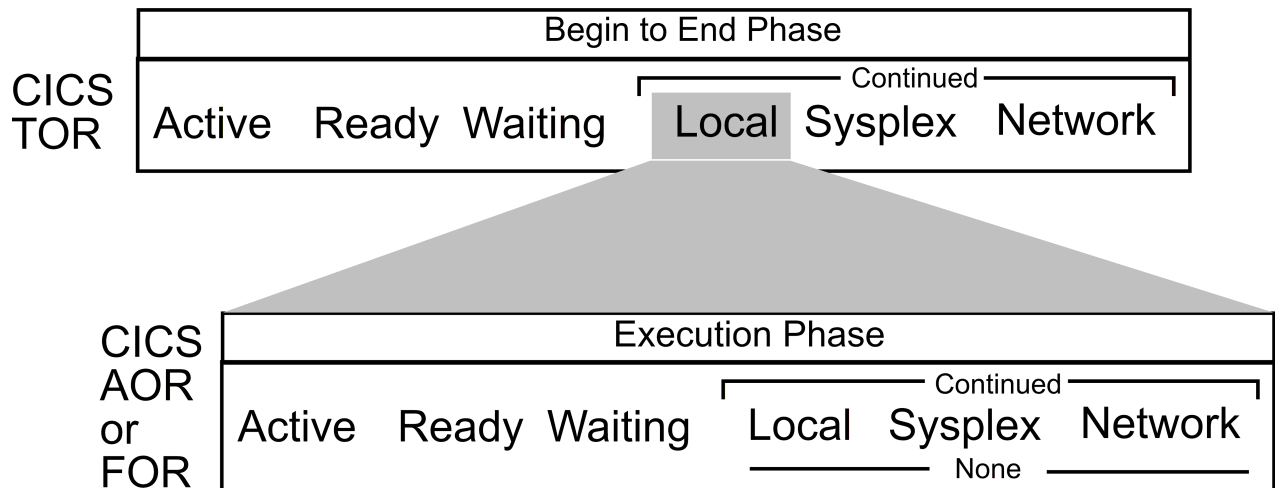
Figure 24. Using states for presenting CICS delay information
