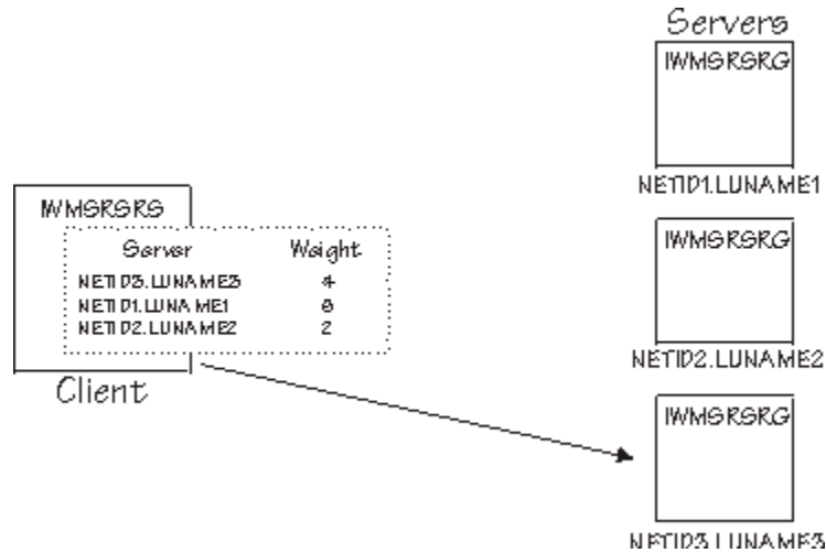
Figure 23. Example of using sysplex routing services
