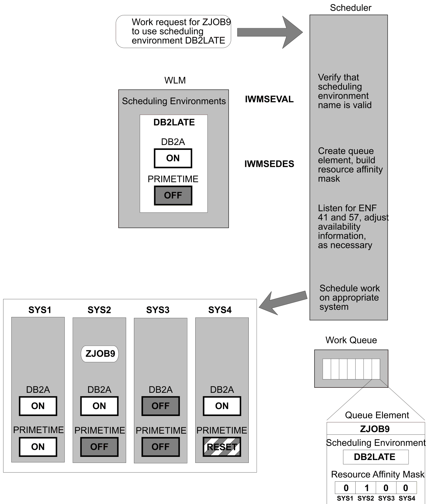
Figure 22. Scheduling environment flow
