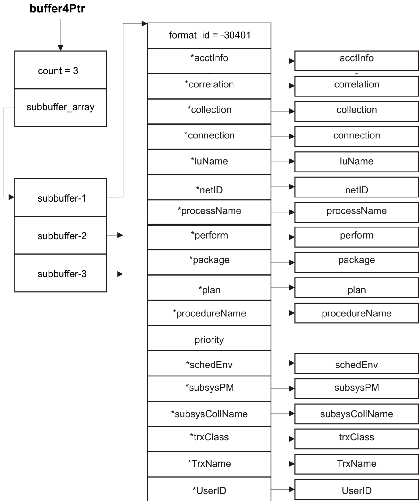
Figure 14. Sub-buffer arm_subbuffer_zos_classify
