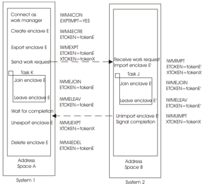
Figure 10. Using a multisystem enclave
