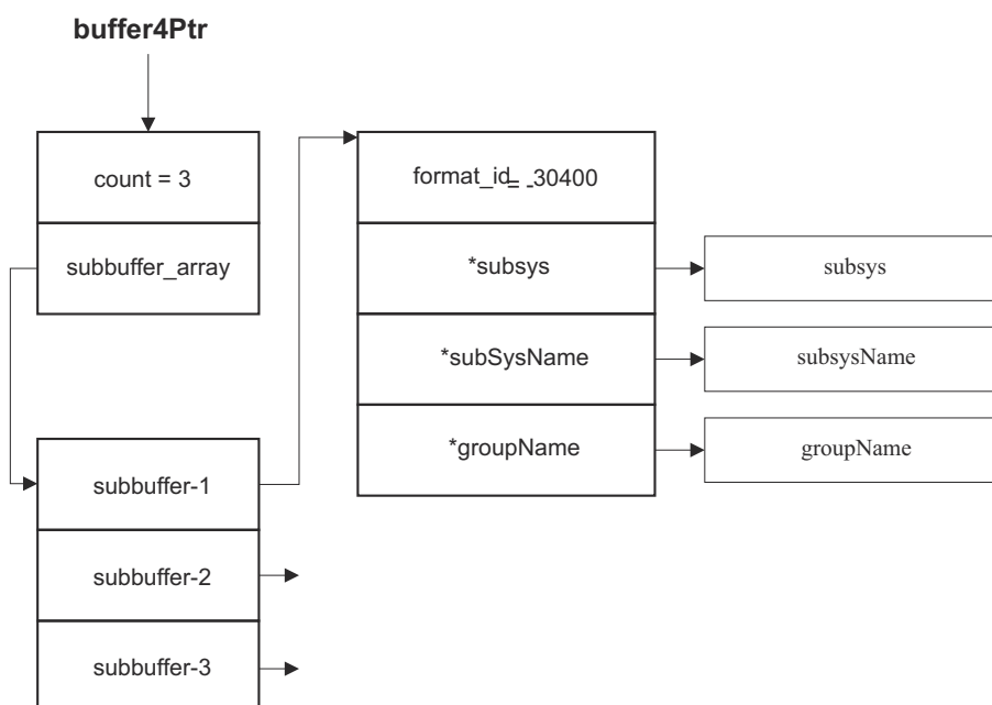
Figure 13. Sub-buffer arm_subbuffer_zos_connect_t
