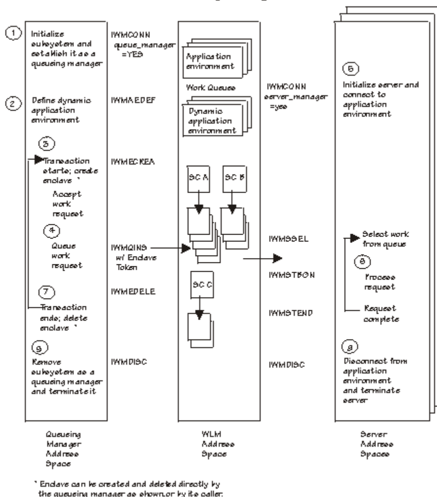
Figure 17. Services for a queueing manager
