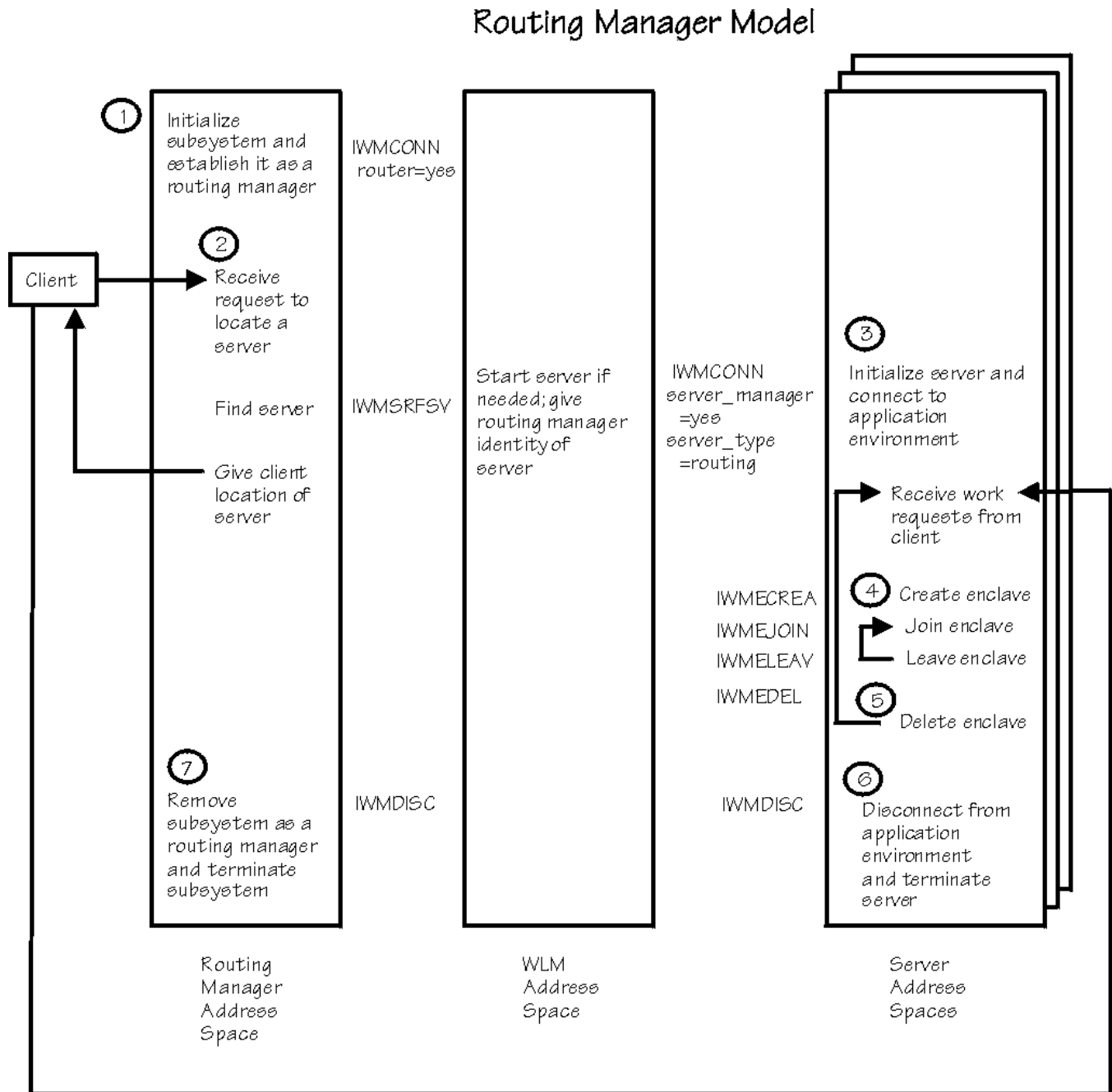
Figure 19. Example of routing manager services
