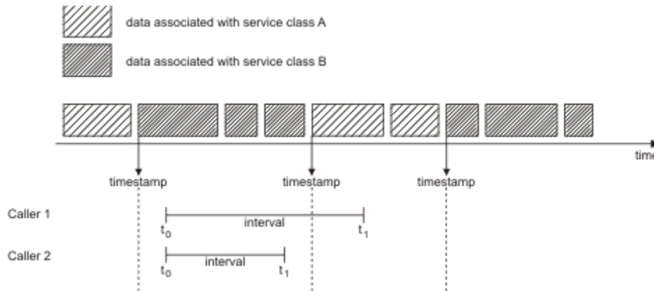
Figure 28. Mixed-class-indication timestamp in relation to the time interval
