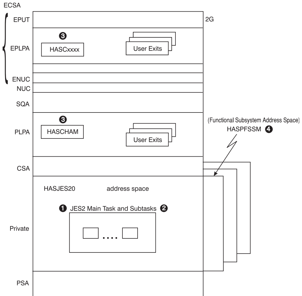
Figure 4. JES2 and FSS Address Spaces
