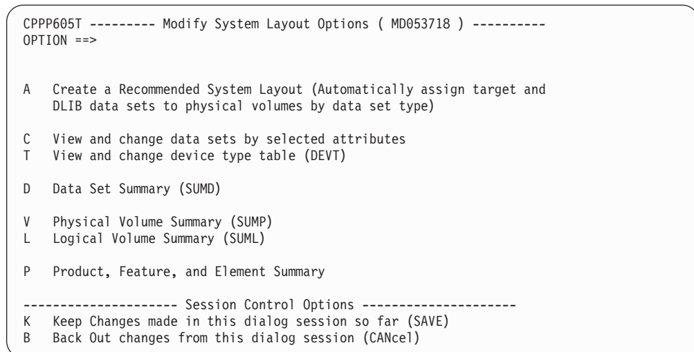
Figure 61. Panel: Modify system layout options
