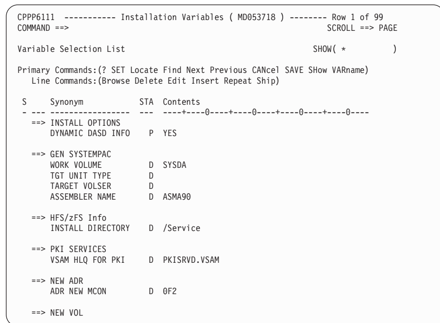
Figure 39. Panel: Variable selection list - variable synonyms
