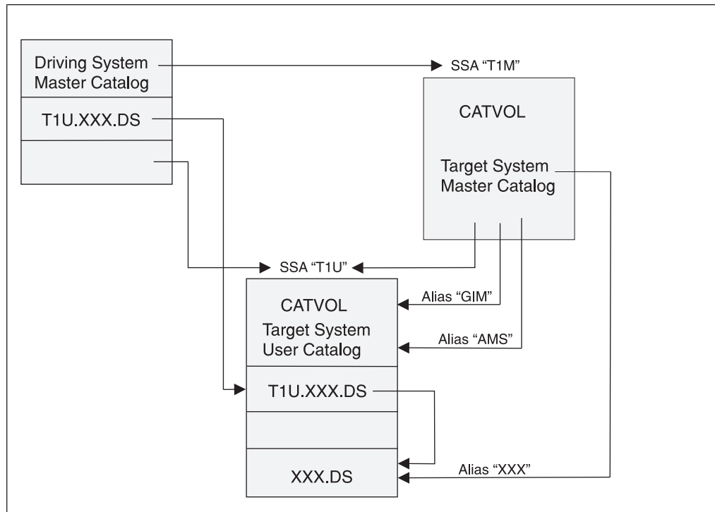
Figure 127. Default catalog structure for full system replacement
