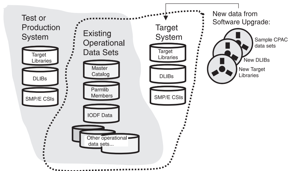
Figure 32. Software upgrade option preserves your existing operational data
