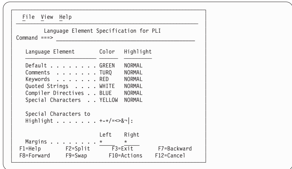
Figure 7. HILITE Language Element Specification Screen (ISREPC1)
