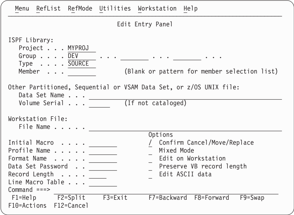
Figure 2. Edit Entry panel (ISREDM01)
