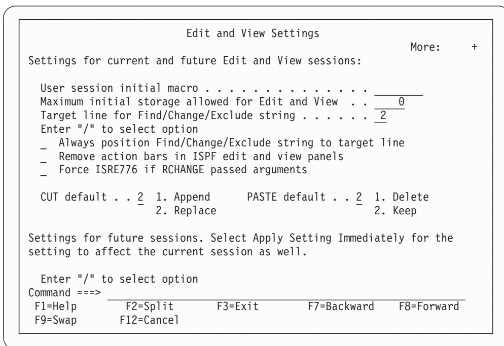
Figure 122. Edit and View Settings panel (ISREDSSET)
