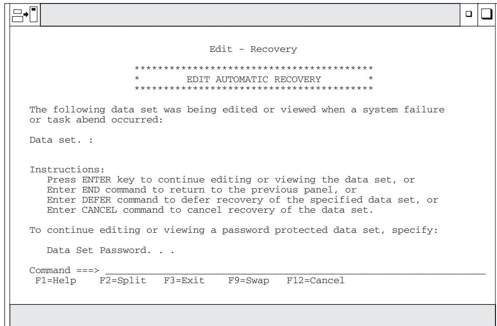
Figure 10. Edit Recovery panel (ISREDM02)
