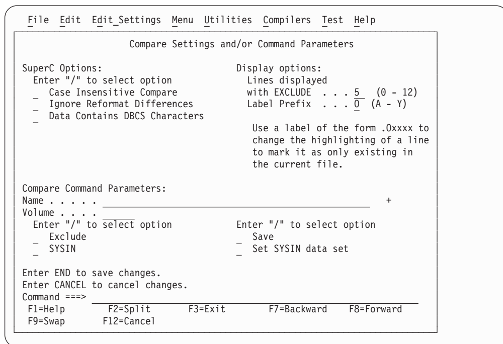
Figure 110. Edit Compare Settings and/or Command Parameters panel
