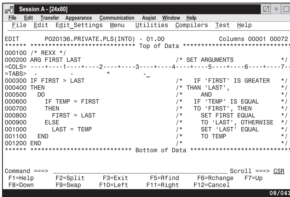
Figure 96. TAB line command example. A =TABS> line with four software tabs and one hardware tab defined.
