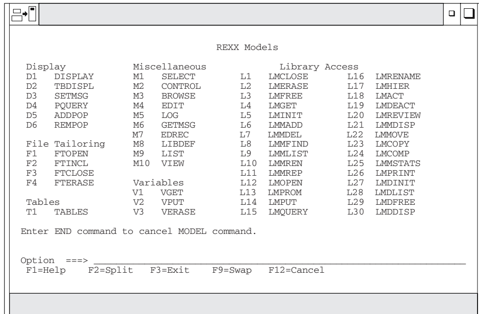
Figure 135. REXX Models panel (ISREMRXC)
